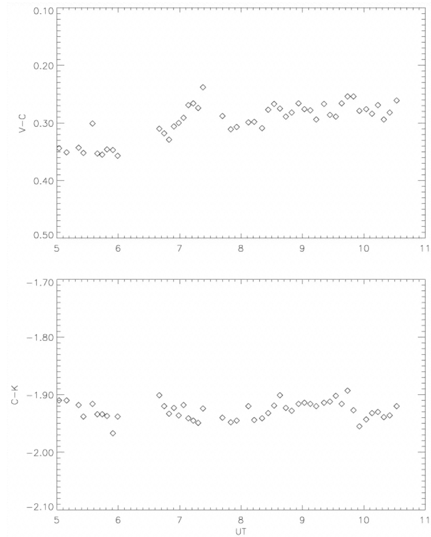
Fig. 4. from The Timescales of the Optical Variability of Blazars. V. 3C 371 Carini, Noble, & Miller 1998 AJ 116 2667 doi:10.1086/300656 https://dx.doi.org/10.1086/300656 © 1998. The American Astronomical Society. All rights reserved. Printed in U.S.A.
