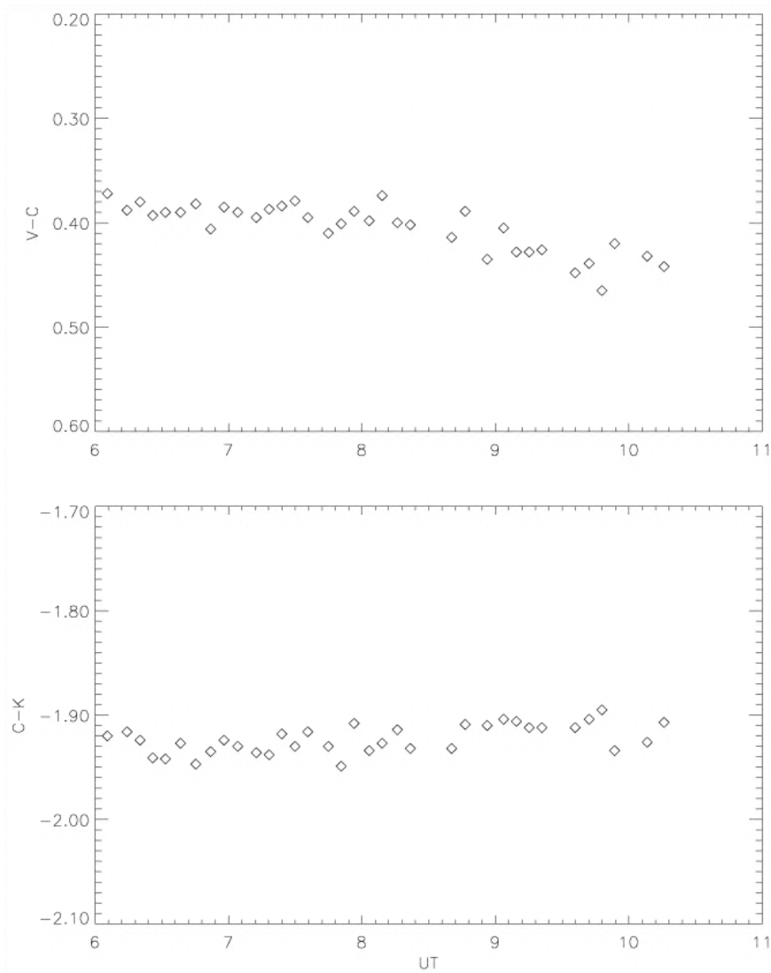
Fig. 2. from The Timescales of the Optical Variability of Blazars. V. 3C 371 Carini, Noble, & Miller 1998 AJ 116 2667 doi:10.1086/300656 https://dx.doi.org/10.1086/300656 © 1998. The American Astronomical Society. All rights reserved. Printed in U.S.A.
