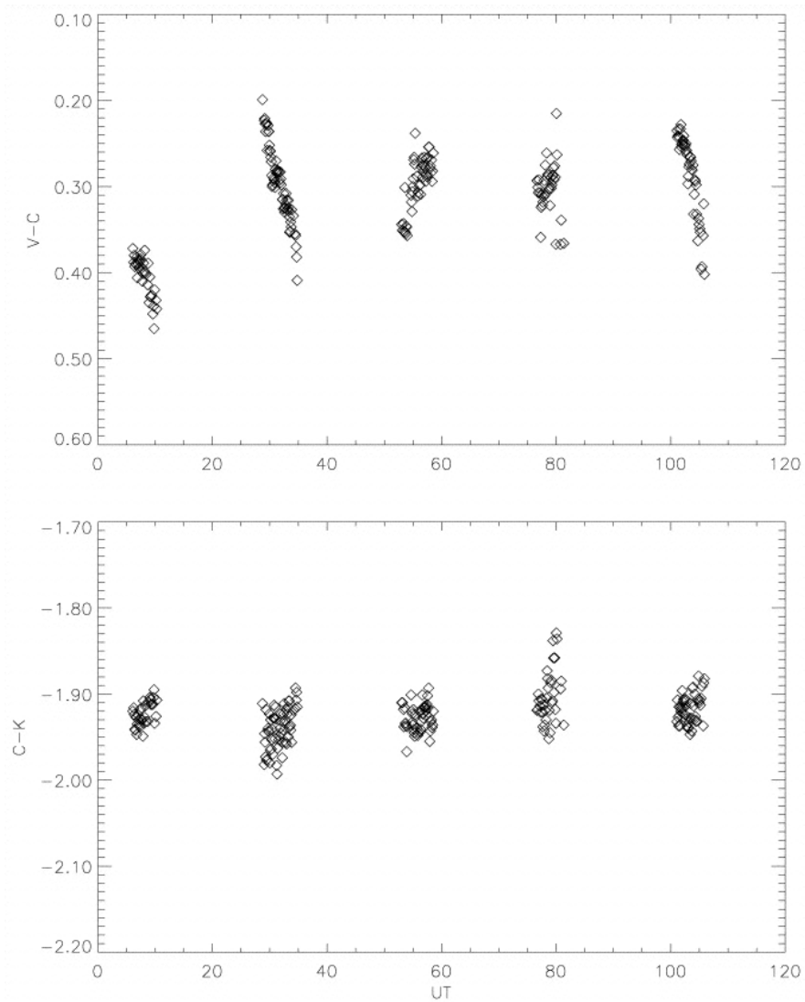
Fig. 1. from The Timescales of the Optical Variability of Blazars. V. 3C 371 Carini, Noble, & Miller 1998 AJ 116 2667 doi:10.1086/300656 https://dx.doi.org/10.1086/300656 © 1998. The American Astronomical Society. All rights reserved. Printed in U.S.A.
