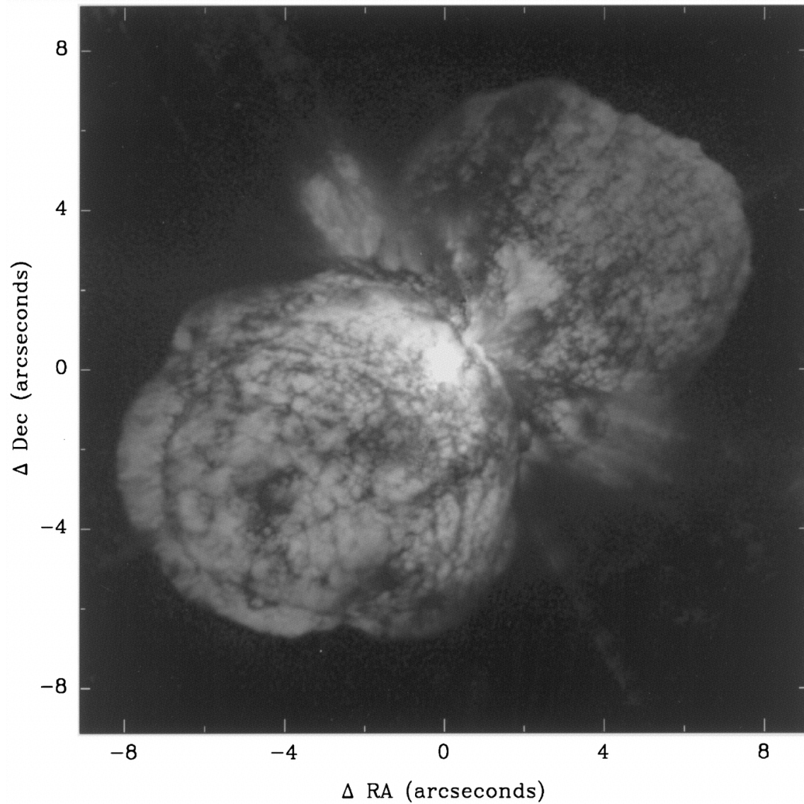
Fig. 2. from Hubble Space Telescope Wide Field Planetary Camera 2 Observations of Carinae Morse et al. 1998 AJ 116 2443 doi:10.1086/300581 https://dx.doi.org/10.1086/300581 © 1998. The American Astronomical Society. All rights reserved. Printed in U.S.A.
