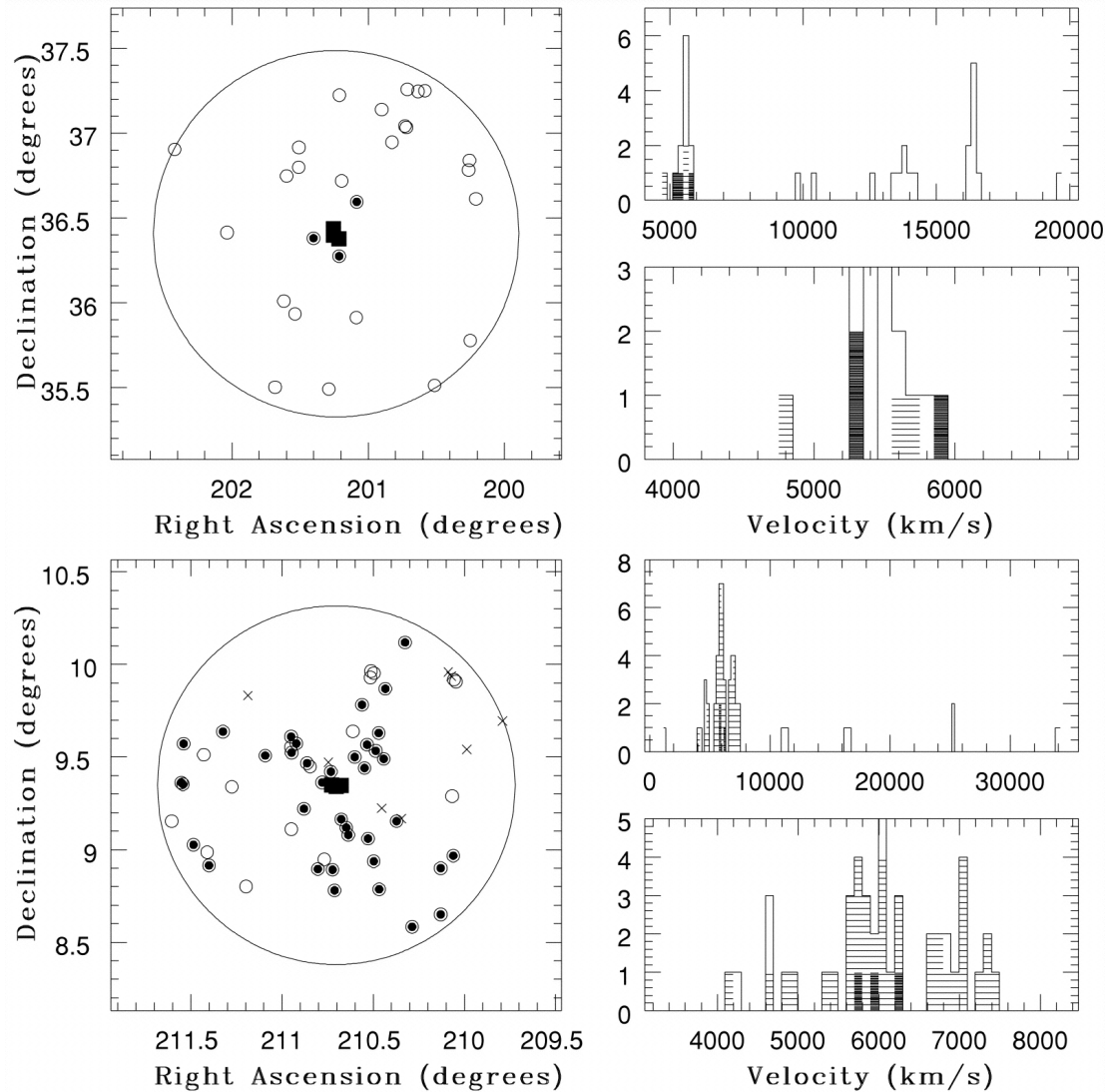
Fig. 9. from Environments of Redshift Survey Compact Groups of Galaxies Barton, de Carvalho, & Geller 1998 AJ 116 1573 doi:10.1086/300531 https://dx.doi.org/10.1086/300531 © 1998. The American Astronomical Society. All rights reserved. Printed in U.S.A.
