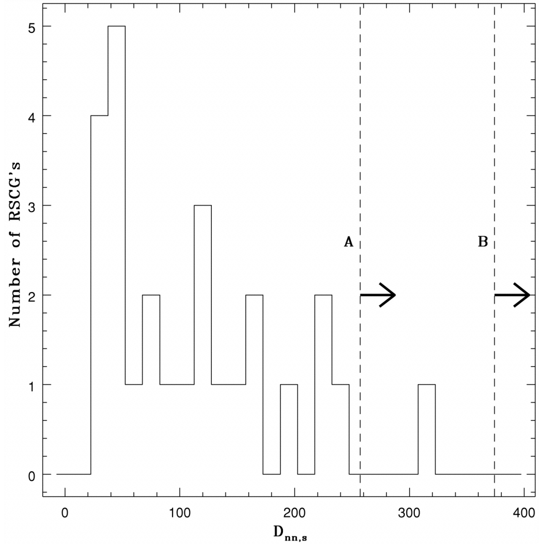
Fig. 2. from Environments of Redshift Survey Compact Groups of Galaxies Barton, de Carvalho, & Geller 1998 AJ 116 1573 doi:10.1086/300531 https://dx.doi.org/10.1086/300531 © 1998. The American Astronomical Society. All rights reserved. Printed in U.S.A.
