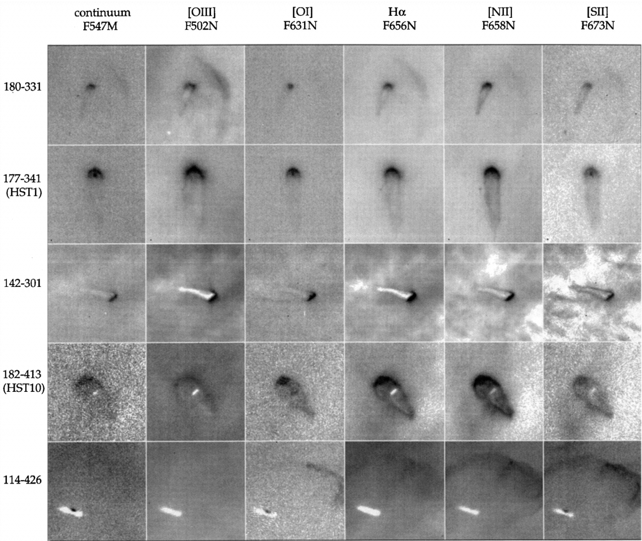
Fig. 7. from Externally Illuminated Young Stellar Environments in the Orion Nebula: Hubble Space Telescope Planetary Camera and Ultraviolet Observations Bally et al. 1998 AJ 116 293 doi:10.1086/300399 https://dx.doi.org/10.1086/300399 © 1998. The American Astronomical Society. All rights reserved. Printed in U.S.A.
