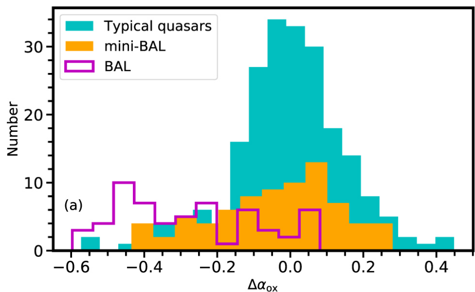
Figure 1. from Long-timescale X-Ray Variability of BAL and Mini-BAL Quasars null 2020 RNAAS 4 168 doi:10.3847/2515-5172/abbb8c https://dx.doi.org/10.3847/2515-5172/abbb8c © 2020. The American Astronomical Society. All rights reserved.
