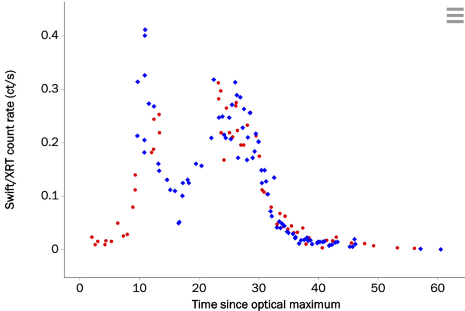
Figure 1. from Similarities between the X-Ray Light Curves of the 2016 and 2020 Eruptions of the Recurrent Nova LMC 1968 null 2020 RNAAS 4 142 doi:10.3847/2515-5172/abae72 https://dx.doi.org/10.3847/2515-5172/abae72 © 2020. The American Astronomical Society. All rights reserved.
