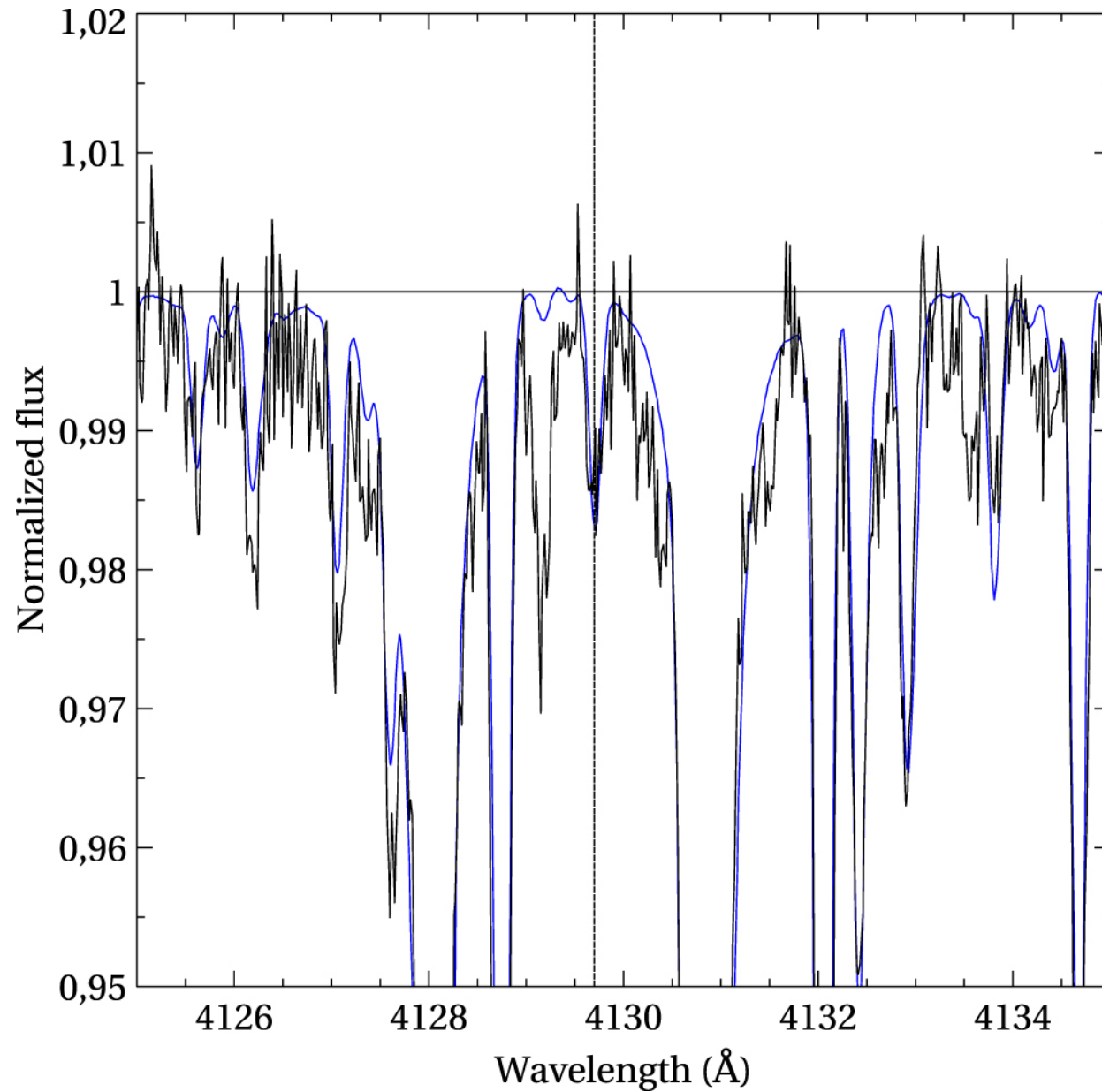
Figure 1. from The Abundance of Europium in HR 6096 A null 2019 RNAAS 3 167 doi:10.3847/2515-5172/ab5441 https://dx.doi.org/10.3847/2515-5172/ab5441 © 2019. The American Astronomical Society. All rights reserved.
