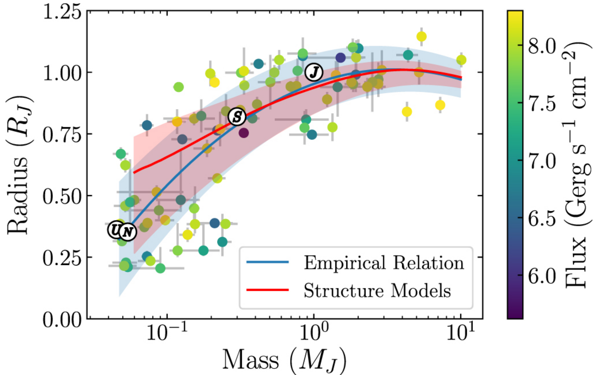
Figure 1. from An Empirical Mass–Radius Relation for Cool Giant Planets null 2019 RNAAS 3 128 doi:10.3847/2515-5172/ab4353 https://dx.doi.org/10.3847/2515-5172/ab4353 © 2019. The American Astronomical Society. All rights reserved.
