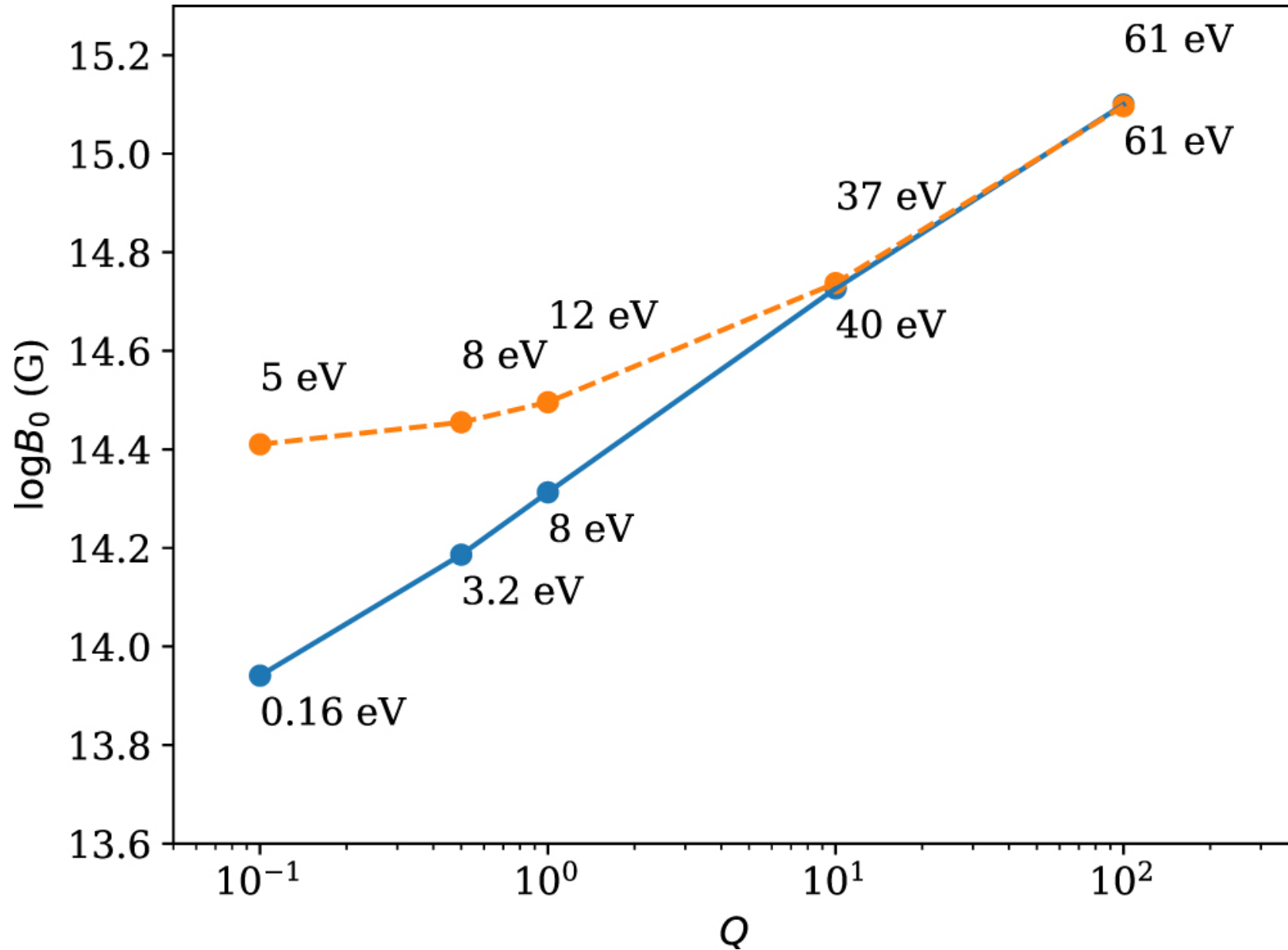
Figure 1. from Is PSR J0250+5854 at the Hall Attractor Stage? null 2018 RNAAS 2 171 doi:10.3847/2515-5172/aae207 https://dx.doi.org/10.3847/2515-5172/aae207 © 2018. The American Astronomical Society. All rights reserved.
