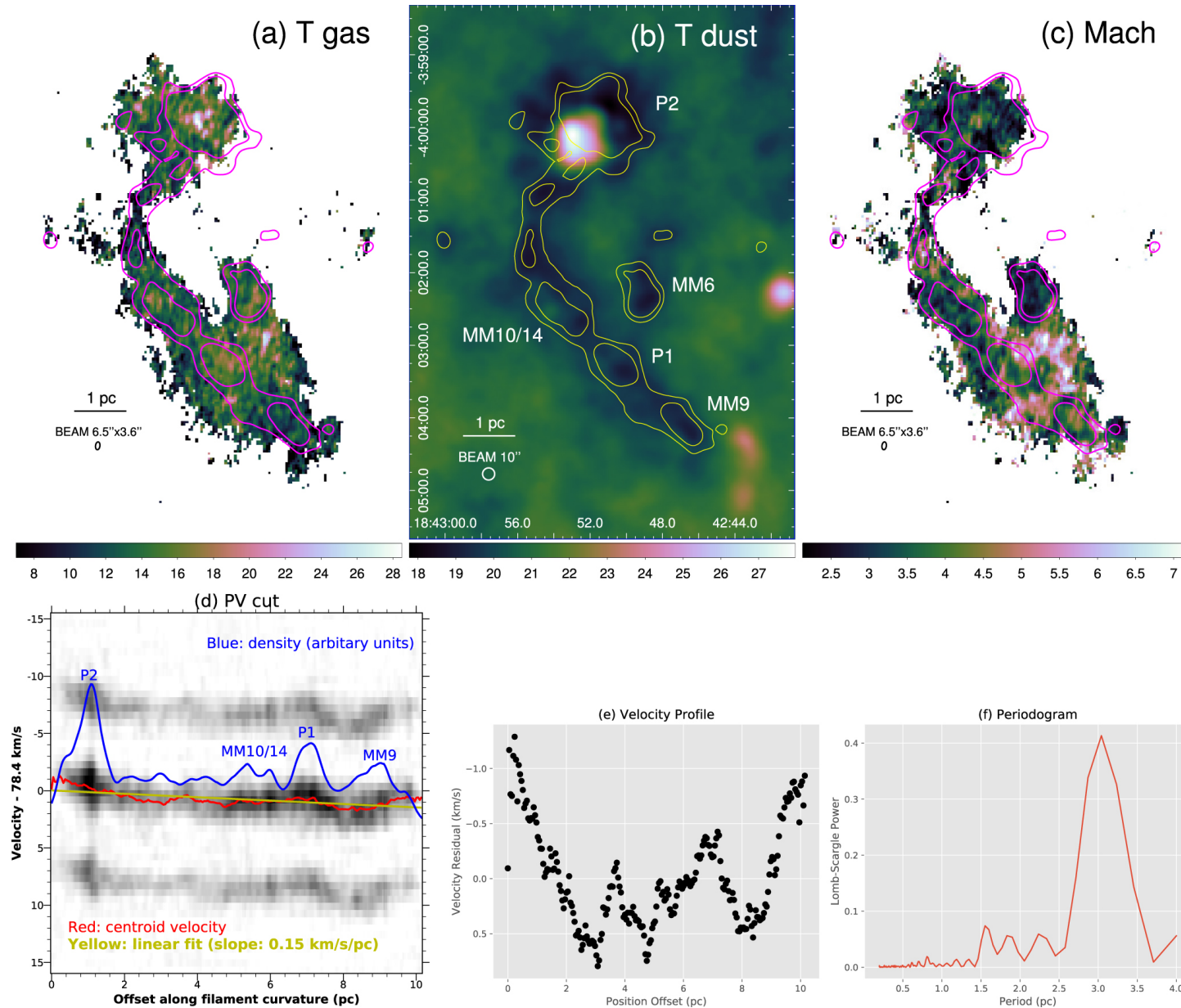
Figure 1. from Temperature, Turbulence, and Kinematics of the Giant Filamentary Infrared Dark Cloud G28.34+0.06 at 0.1pc Resolution null 2018 RNAAS 2 52 doi:10.3847/2515-5172/aacb29 https://dx.doi.org/10.3847/2515-5172/aacb29 © 2018. The American Astronomical Society. All rights reserved.
