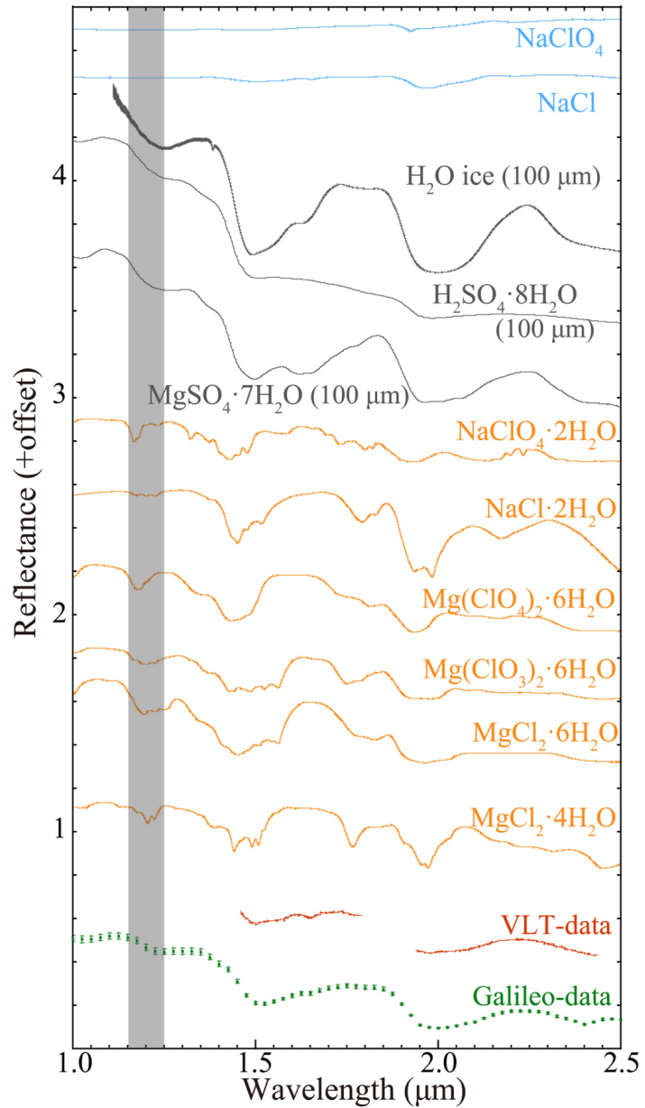
Figure 1. from Shuya Tan et al 2022 Planet. Sci. J. 3 doi:10.3847/PSJ/ac596c http://dx.doi.org/10.3847/PSJ/ac596c © 2022. The Author(s). Published by the American Astronomical Society.
