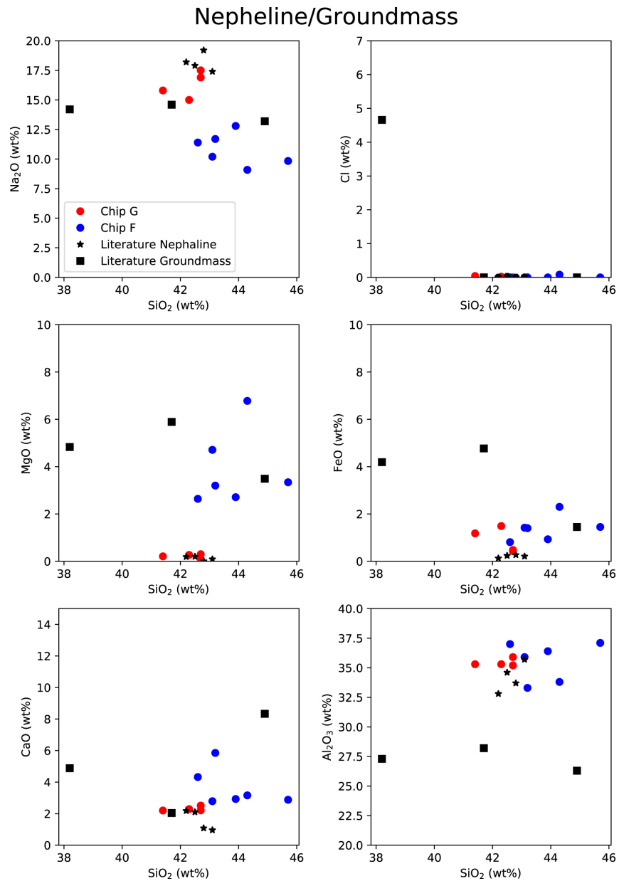
Figure 6. from Volatility of Sodium in Carbonaceous Chondrites at Temperatures Consistent with Low-perihelion Asteroids null 2021 PSJ 2 165 doi:10.3847/PSJ/ac0d02 https://dx.doi.org/10.3847/PSJ/ac0d02 © 2021. The Author(s). Published by the American Astronomical Society.
