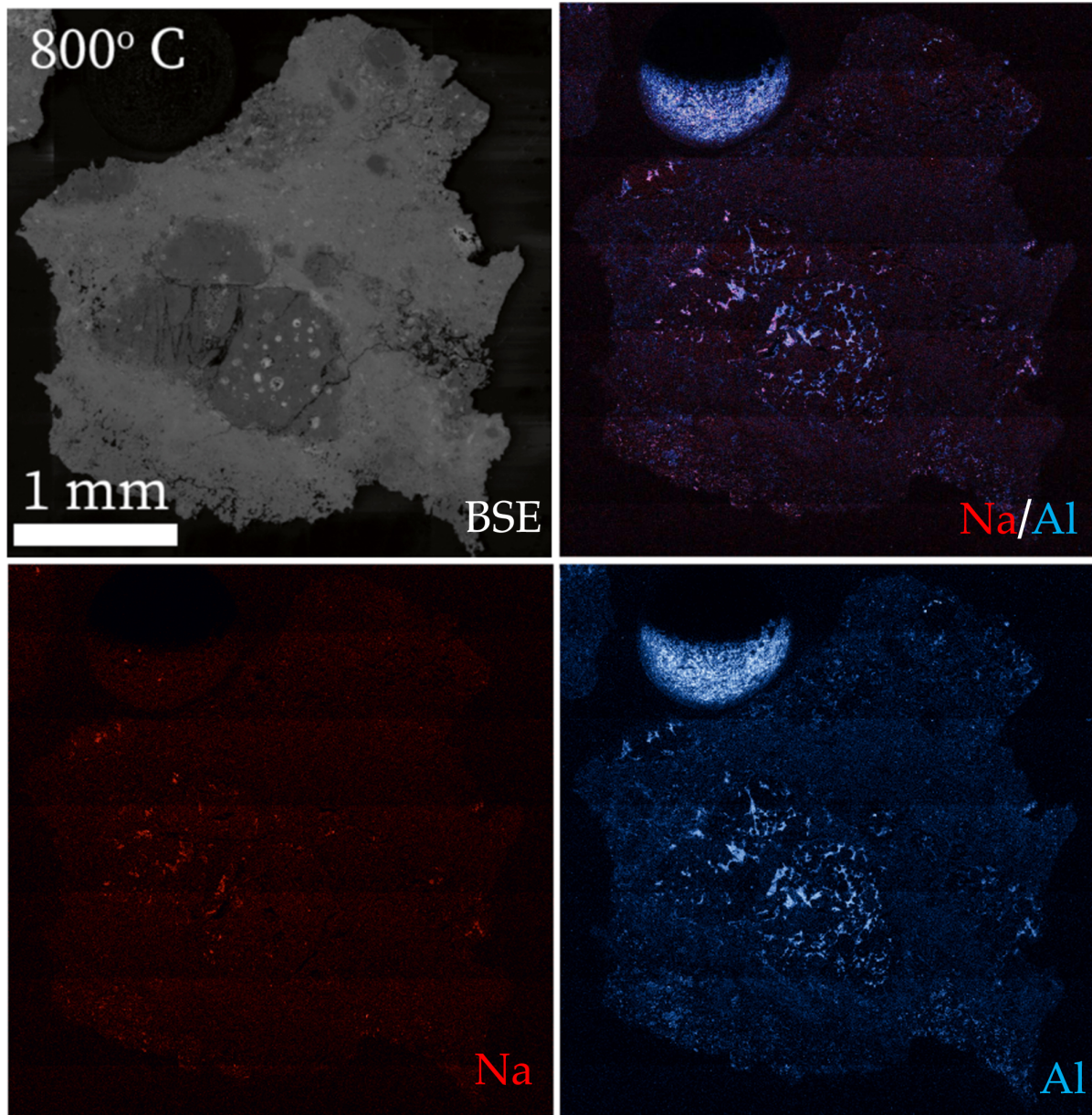
Figure 4. from Volatility of Sodium in Carbonaceous Chondrites at Temperatures Consistent with Low-perihelion Asteroids null 2021 PSJ 2 165 doi:10.3847/PSJ/ac0d02 https://dx.doi.org/10.3847/PSJ/ac0d02 © 2021. The Author(s). Published by the American Astronomical Society.
