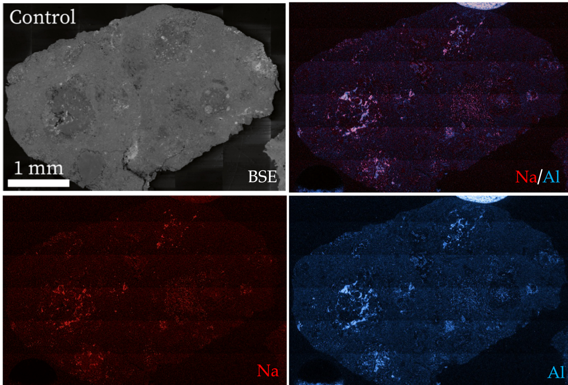
Figure 3. from Volatility of Sodium in Carbonaceous Chondrites at Temperatures Consistent with Low-perihelion Asteroids null 2021 PSJ 2 165 doi:10.3847/PSJ/ac0d02 https://dx.doi.org/10.3847/PSJ/ac0d02 © 2021. The Author(s). Published by the American Astronomical Society.
