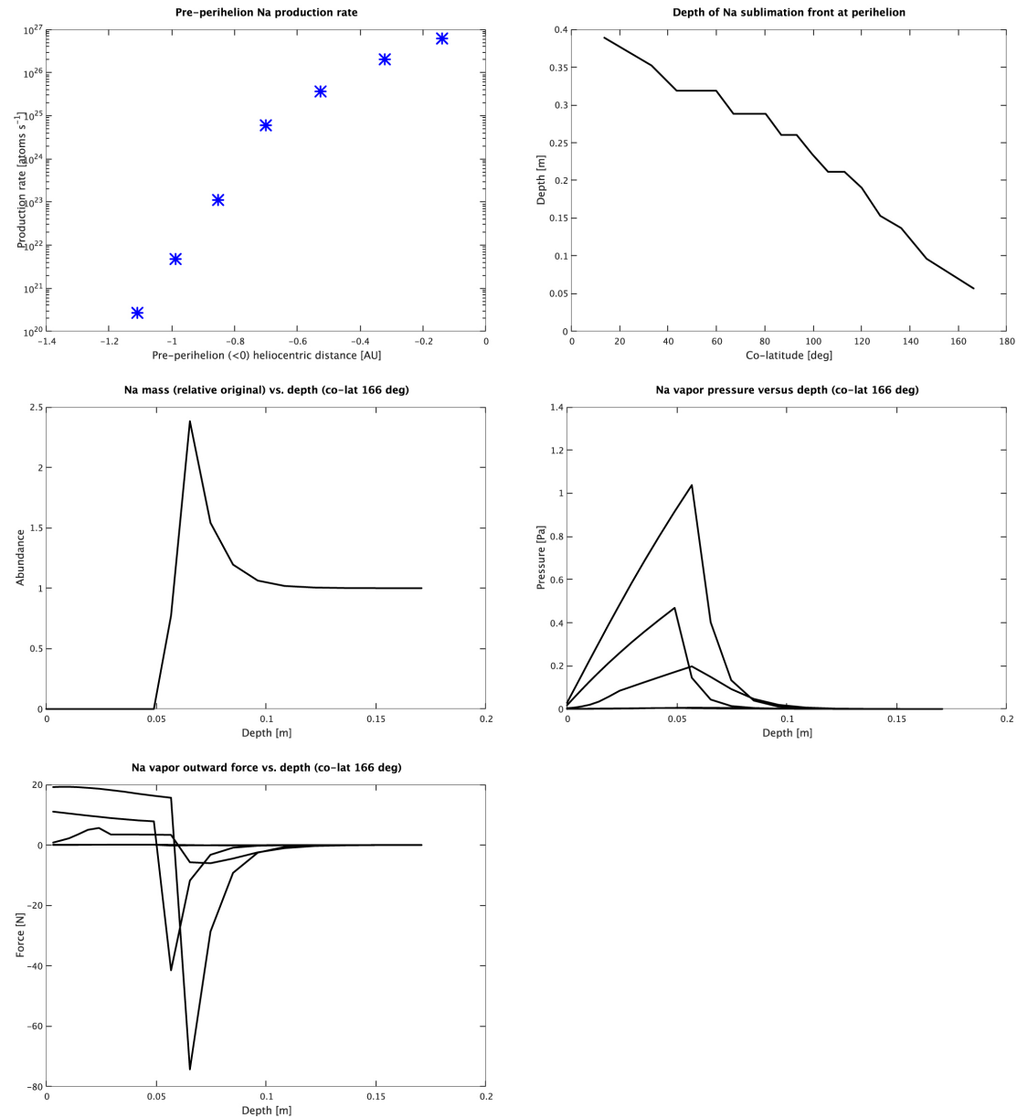
Figure 2. from Volatility of Sodium in Carbonaceous Chondrites at Temperatures Consistent with Low-perihelion Asteroids null 2021 PSJ 2 165 doi:10.3847/PSJ/ac0d02 https://dx.doi.org/10.3847/PSJ/ac0d02 © 2021. The Author(s). Published by the American Astronomical Society.
