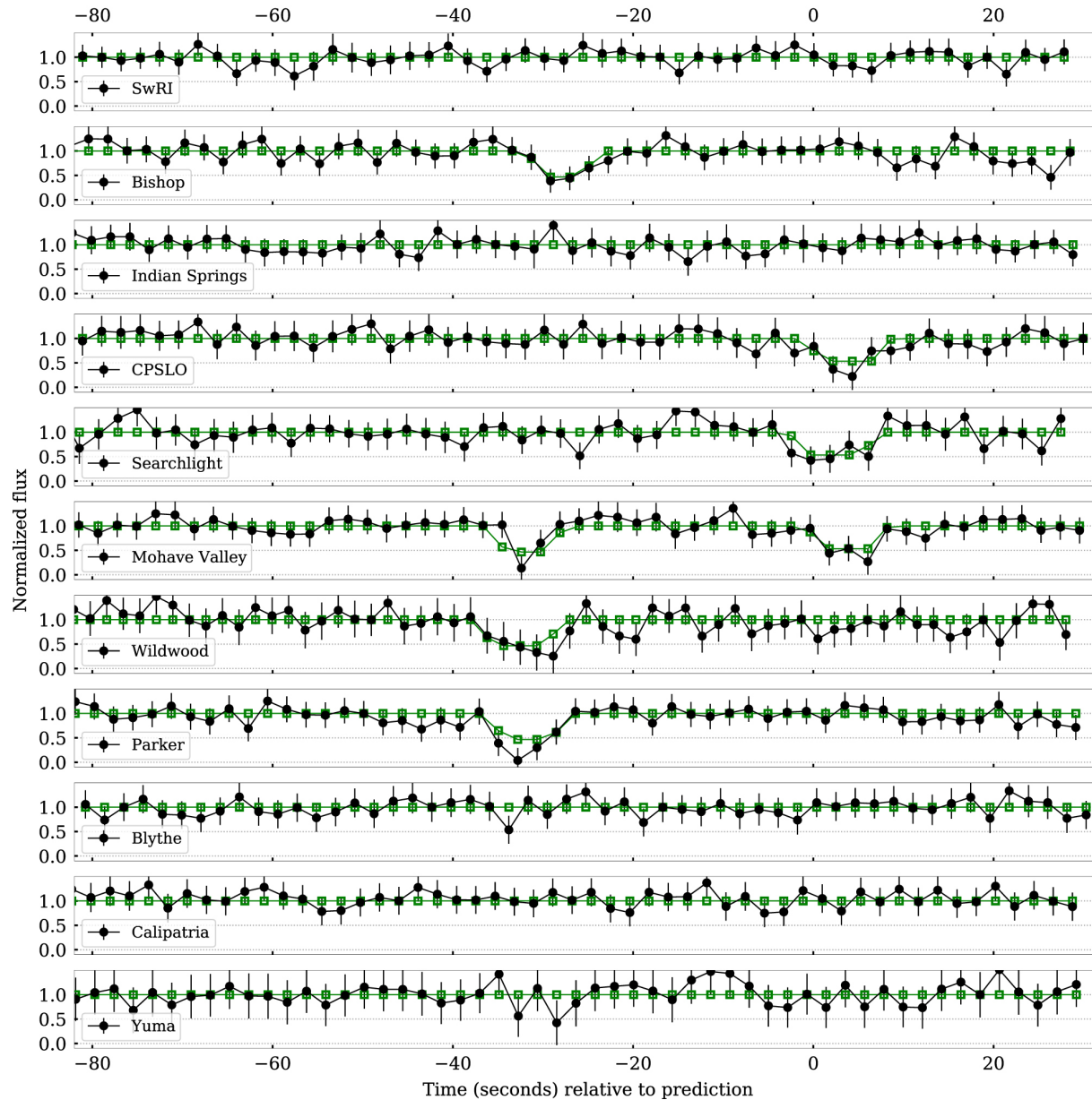
Figure 9. from Stellar Occultation by the Resonant Trans-Neptunian Object (523764) 2014 WC510 Reveals a Close Binary TNO null 2020 PSJ 1 48 doi:10.3847/PSJ/abb23d https://dx.doi.org/10.3847/PSJ/abb23d © 2020. The Author(s). Published by the American Astronomical Society.
