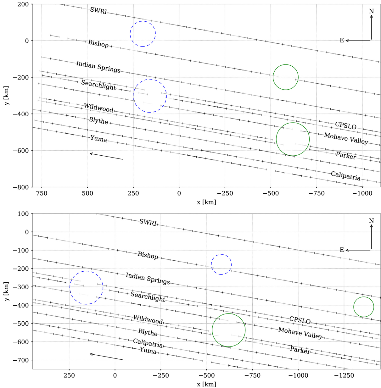
Figure 6. from Stellar Occultation by the Resonant Trans-Neptunian Object (523764) 2014 WC510 Reveals a Close Binary TNO null 2020 PSJ 1 48 doi:10.3847/PSJ/abb23d https://dx.doi.org/10.3847/PSJ/abb23d © 2020. The Author(s). Published by the American Astronomical Society.
