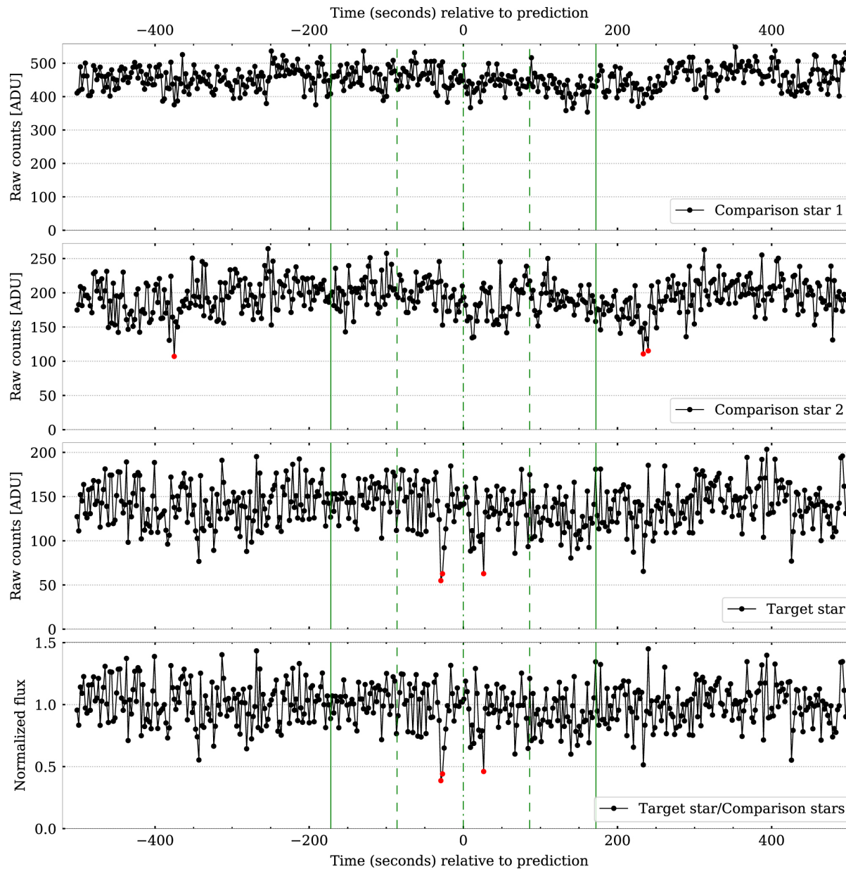
Figure 5. from Stellar Occultation by the Resonant Trans-Neptunian Object (523764) 2014 WC510 Reveals a Close Binary TNO null 2020 PSJ 1 48 doi:10.3847/PSJ/abb23d https://dx.doi.org/10.3847/PSJ/abb23d © 2020. The Author(s). Published by the American Astronomical Society.
