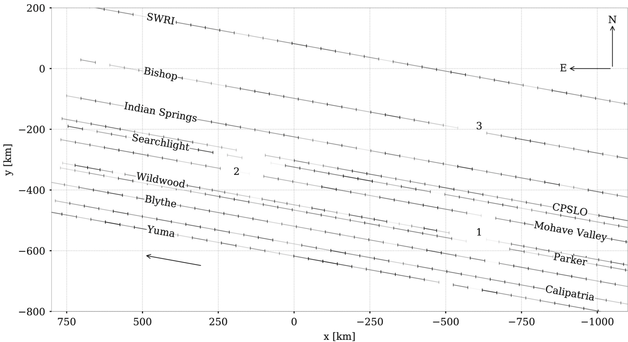
Figure 4. from Stellar Occultation by the Resonant Trans-Neptunian Object (523764) 2014 WC510 Reveals a Close Binary TNO null 2020 PSJ 1 48 doi:10.3847/PSJ/abb23d https://dx.doi.org/10.3847/PSJ/abb23d © 2020. The Author(s). Published by the American Astronomical Society.
