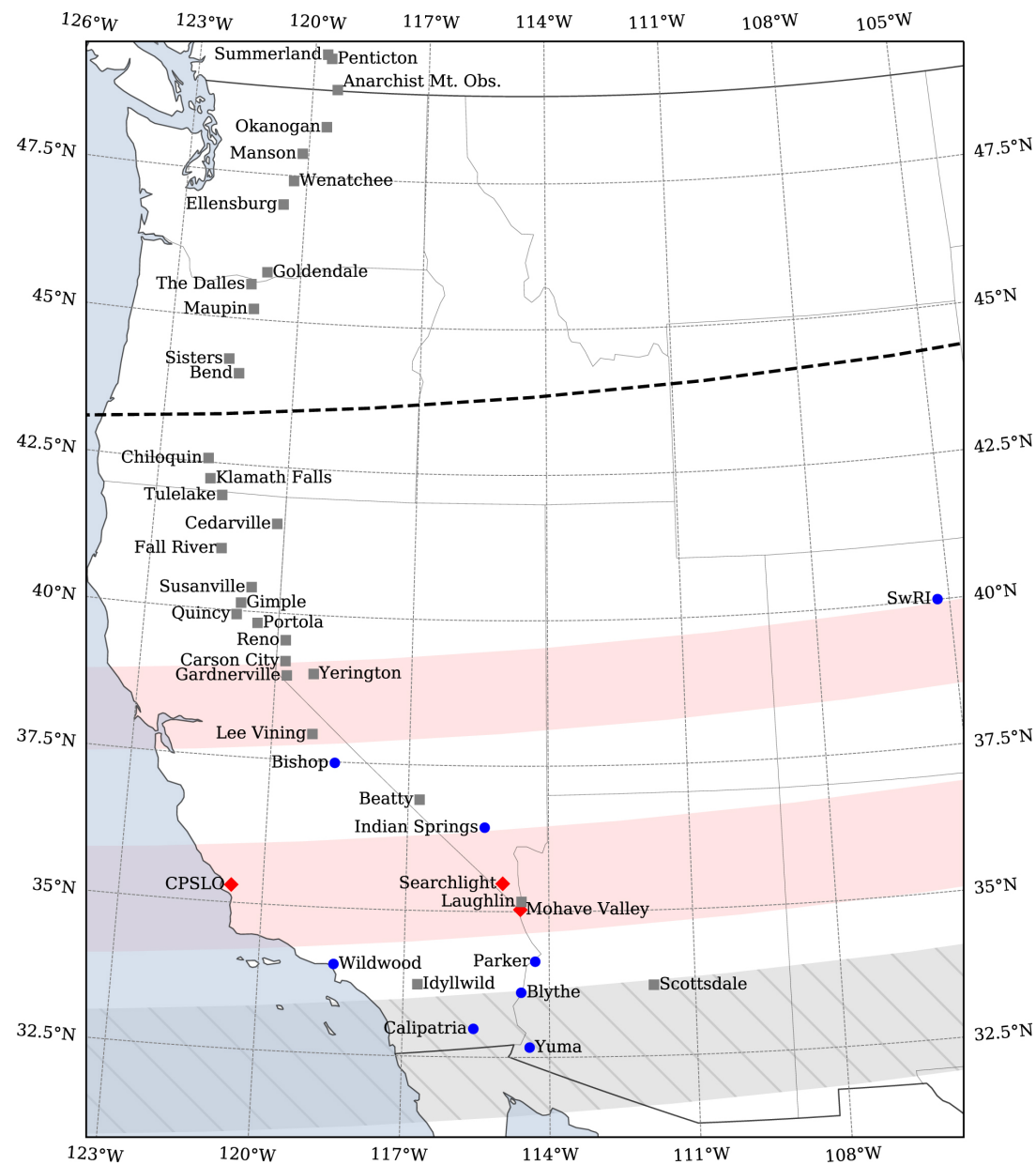
Figure 2. from Stellar Occultation by the Resonant Trans-Neptunian Object (523764) 2014 WC510 Reveals a Close Binary TNO null 2020 PSJ 1 48 doi:10.3847/PSJ/abb23d https://dx.doi.org/10.3847/PSJ/abb23d © 2020. The Author(s). Published by the American Astronomical Society.
