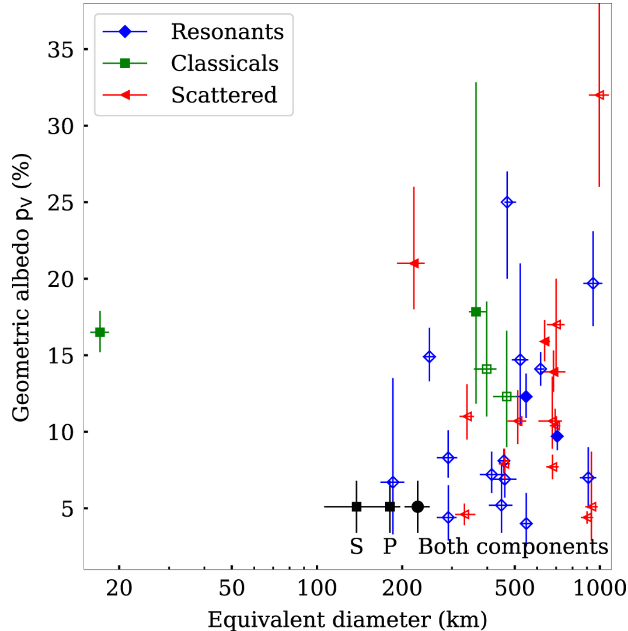
Figure 10. from Stellar Occultation by the Resonant Trans-Neptunian Object (523764) 2014 WC510 Reveals a Close Binary TNO null 2020 PSJ 1 48 doi:10.3847/PSJ/abb23d https://dx.doi.org/10.3847/PSJ/abb23d © 2020. The Author(s). Published by the American Astronomical Society.
