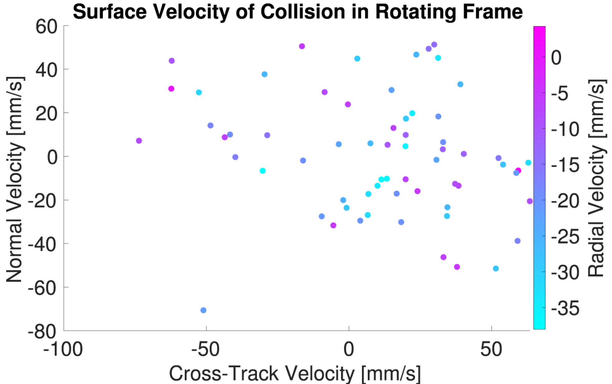
Figure 5. from High-fidelity Modeling of Rotationally Fissioned Asteroids null 2020 PSJ 1 25 doi:10.3847/PSJ/ab9a39 https://dx.doi.org/10.3847/PSJ/ab9a39 © 2020. The Author(s). Published by the American Astronomical Society.
