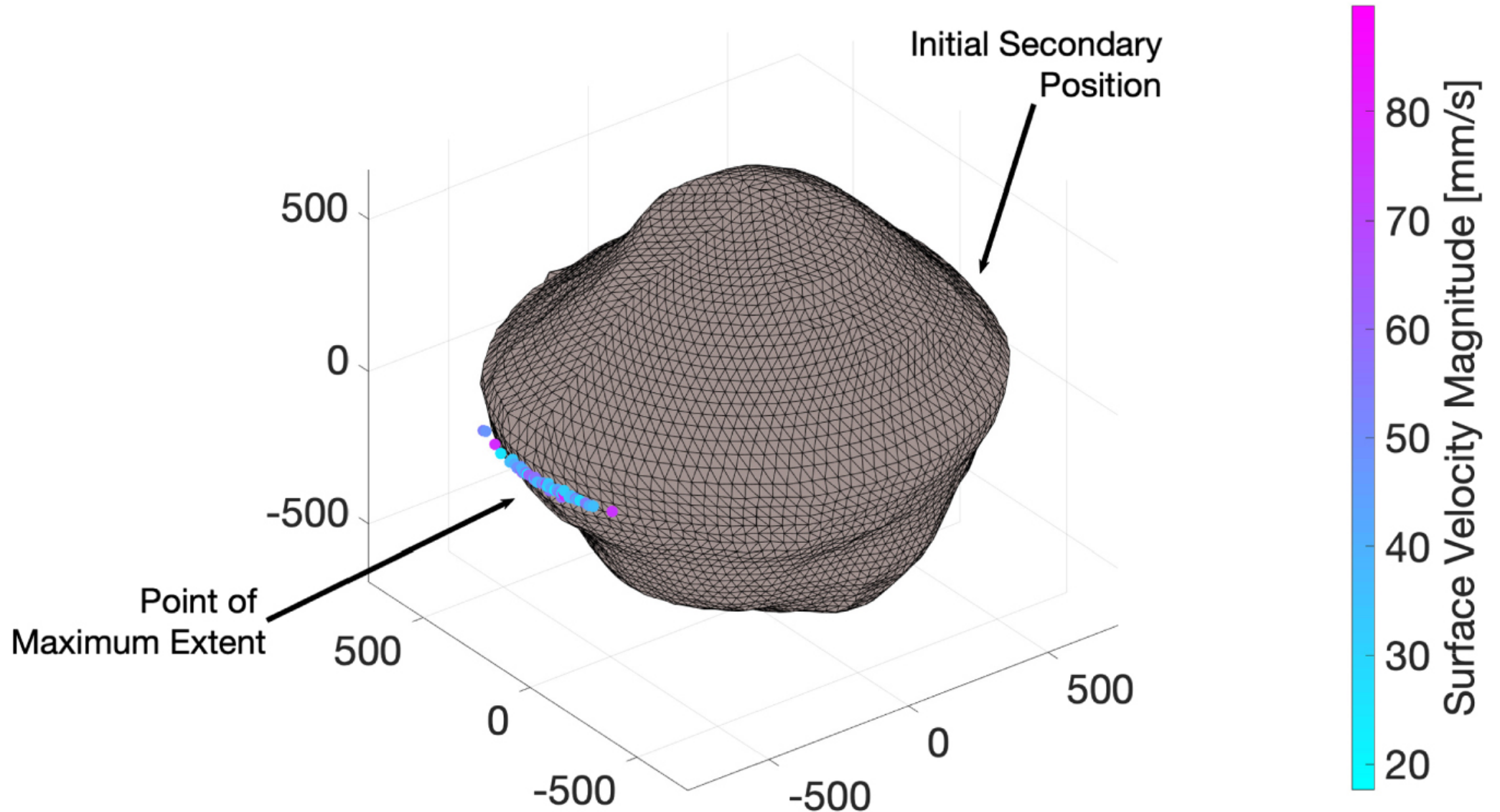
Figure 4. from High-fidelity Modeling of Rotationally Fissioned Asteroids null 2020 PSJ 1 25 doi:10.3847/PSJ/ab9a39 https://dx.doi.org/10.3847/PSJ/ab9a39 © 2020. The Author(s). Published by the American Astronomical Society.
