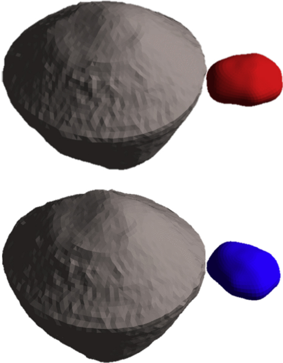
Figure 3. from High-fidelity Modeling of Rotationally Fissioned Asteroids null 2020 PSJ 1 25 doi:10.3847/PSJ/ab9a39 https://dx.doi.org/10.3847/PSJ/ab9a39 © 2020. The Author(s). Published by the American Astronomical Society.
