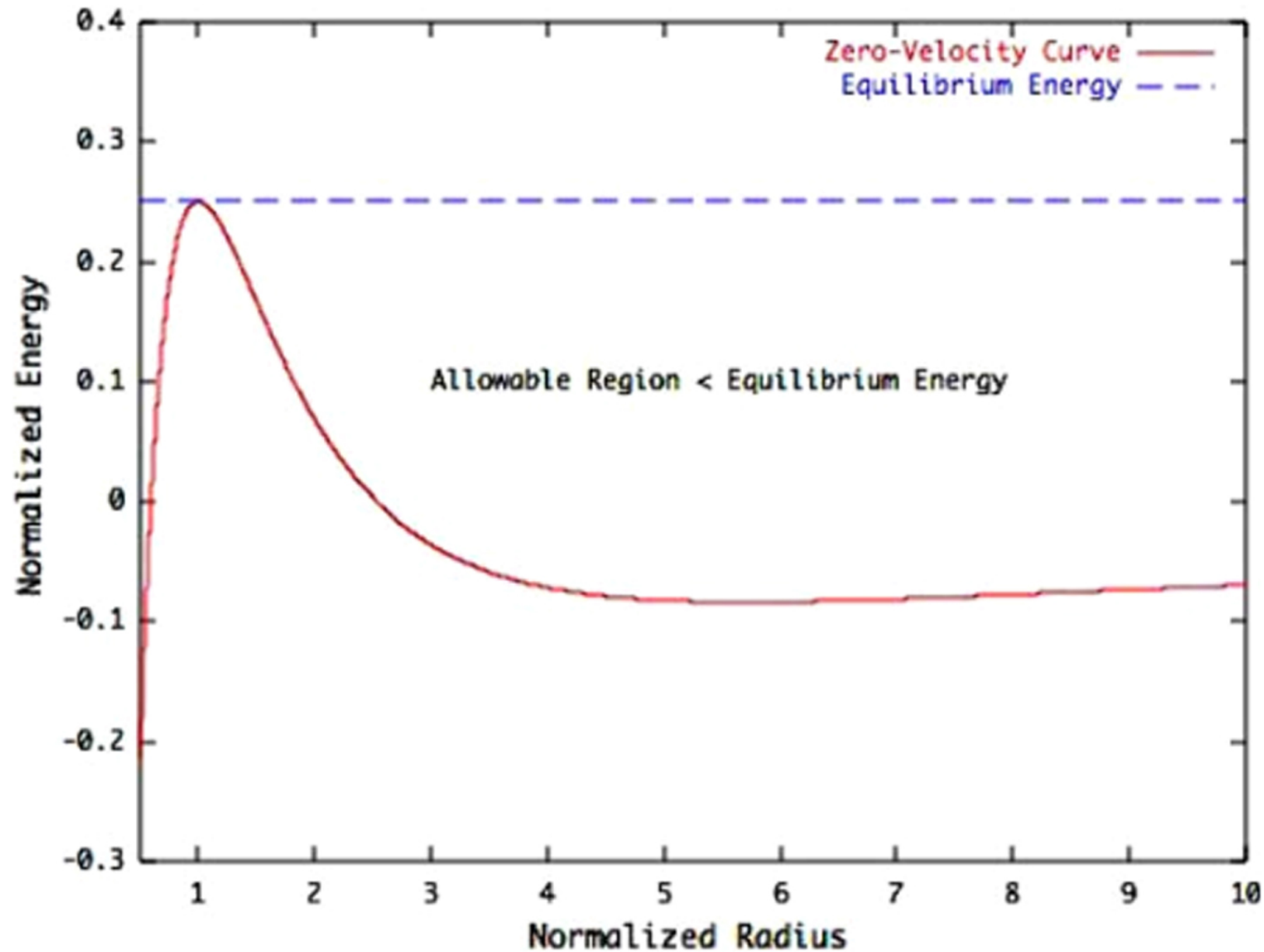
Figure 2. from High-fidelity Modeling of Rotationally Fissioned Asteroids null 2020 PSJ 1 25 doi:10.3847/PSJ/ab9a39 https://dx.doi.org/10.3847/PSJ/ab9a39 © 2020. The Author(s). Published by the American Astronomical Society.
