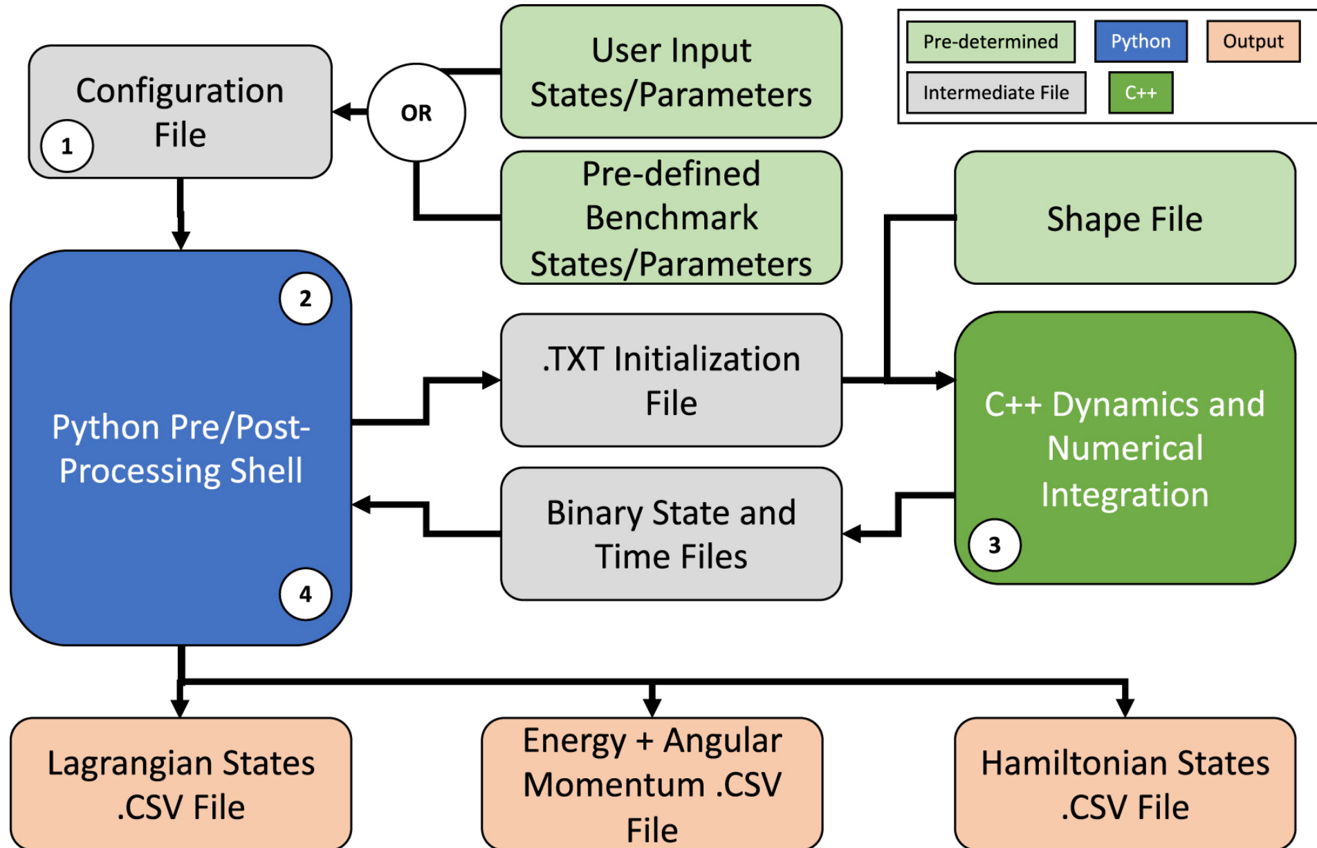
Figure B1. from High-fidelity Modeling of Rotationally Fissioned Asteroids null 2020 PSJ 1 25 doi:10.3847/PSJ/ab9a39 https://dx.doi.org/10.3847/PSJ/ab9a39 © 2020. The Author(s). Published by the American Astronomical Society.
