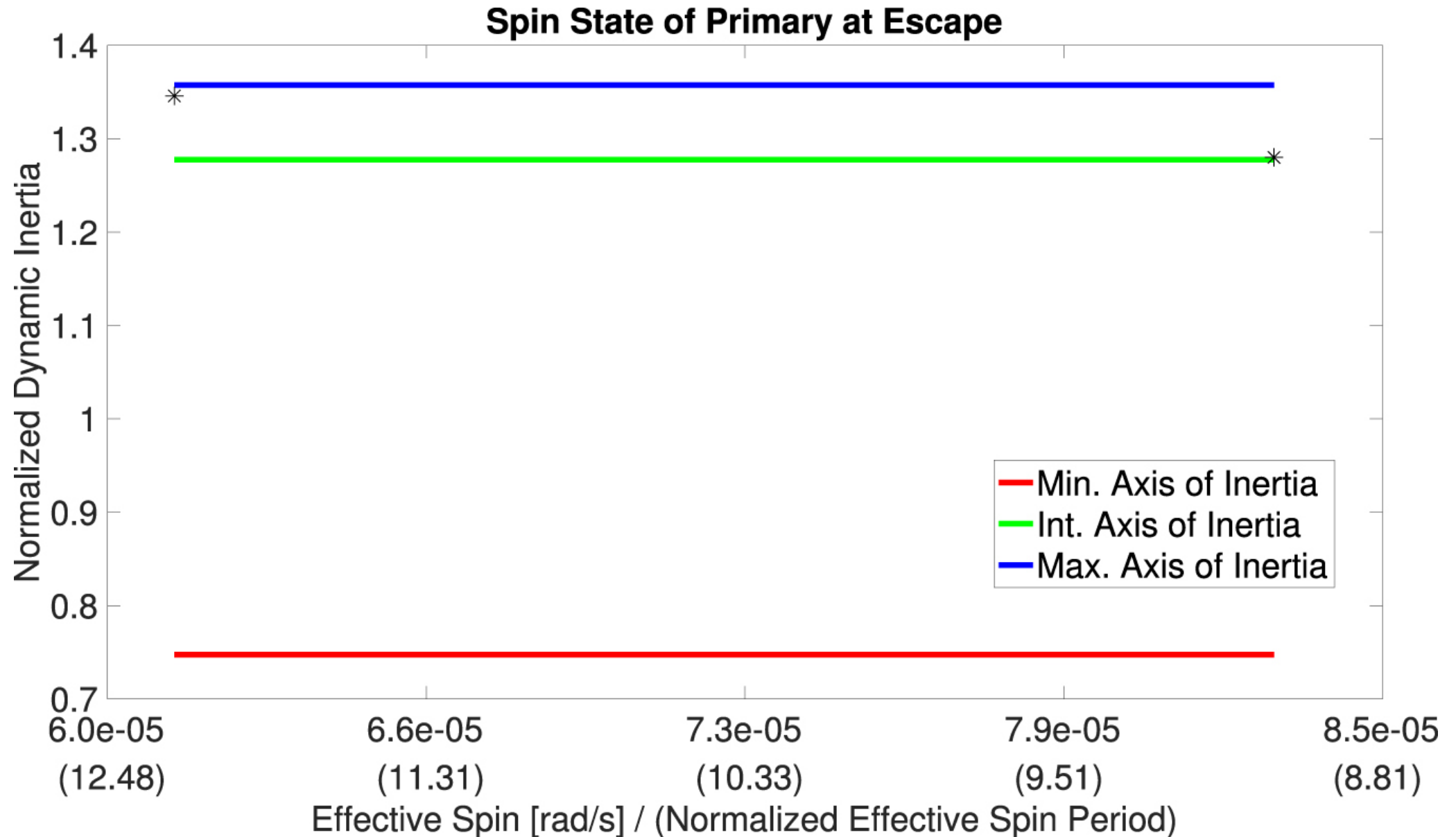
Figure 13. from High-fidelity Modeling of Rotationally Fissioned Asteroids null 2020 PSJ 1 25 doi:10.3847/PSJ/ab9a39 https://dx.doi.org/10.3847/PSJ/ab9a39 © 2020. The Author(s). Published by the American Astronomical Society.
