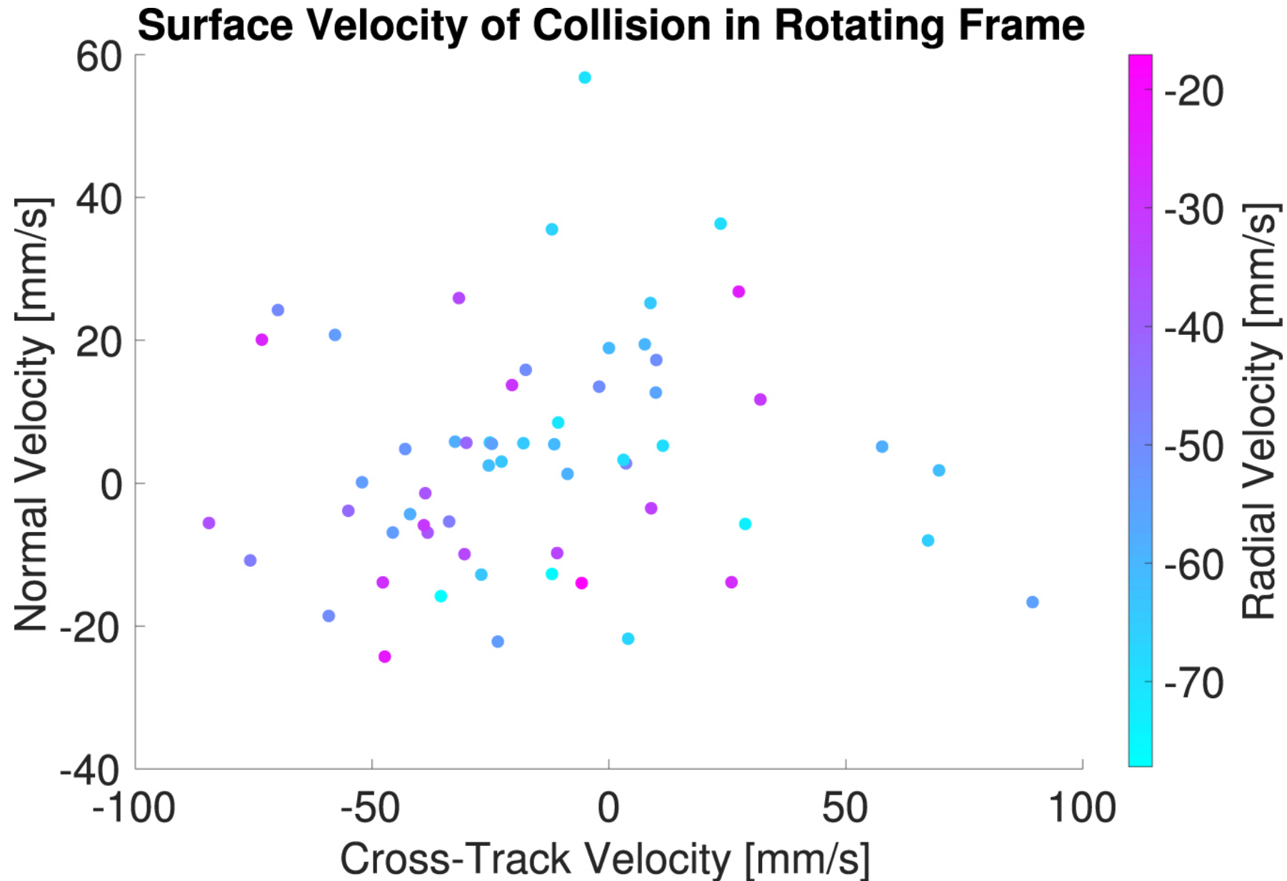
Figure 12. from High-fidelity Modeling of Rotationally Fissioned Asteroids null 2020 PSJ 1 25 doi:10.3847/PSJ/ab9a39 https://dx.doi.org/10.3847/PSJ/ab9a39 © 2020. The Author(s). Published by the American Astronomical Society.
