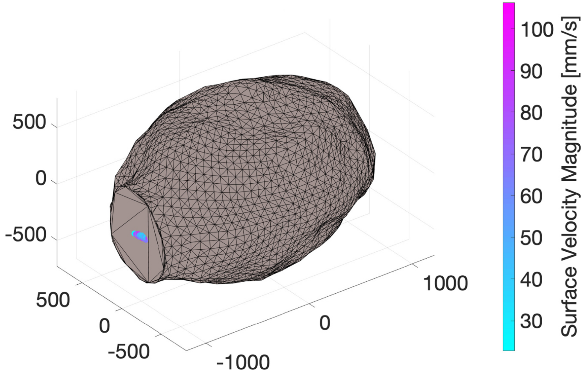
Figure 10. from High-fidelity Modeling of Rotationally Fissioned Asteroids null 2020 PSJ 1 25 doi:10.3847/PSJ/ab9a39 https://dx.doi.org/10.3847/PSJ/ab9a39 © 2020. The Author(s). Published by the American Astronomical Society.
