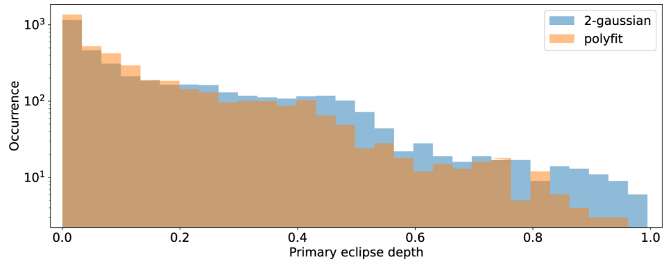
Figure 9. from TESS Eclipsing Binary Stars. I. Short-cadence Observations of 4584 Eclipsing Binaries in Sectors 1–26 null 2022 APJS 258 16 doi:10.3847/1538-4365/ac324a http://dx.doi.org/10.3847/1538-4365/ac324a © 2022. The Author(s). Published by the American Astronomical Society.
