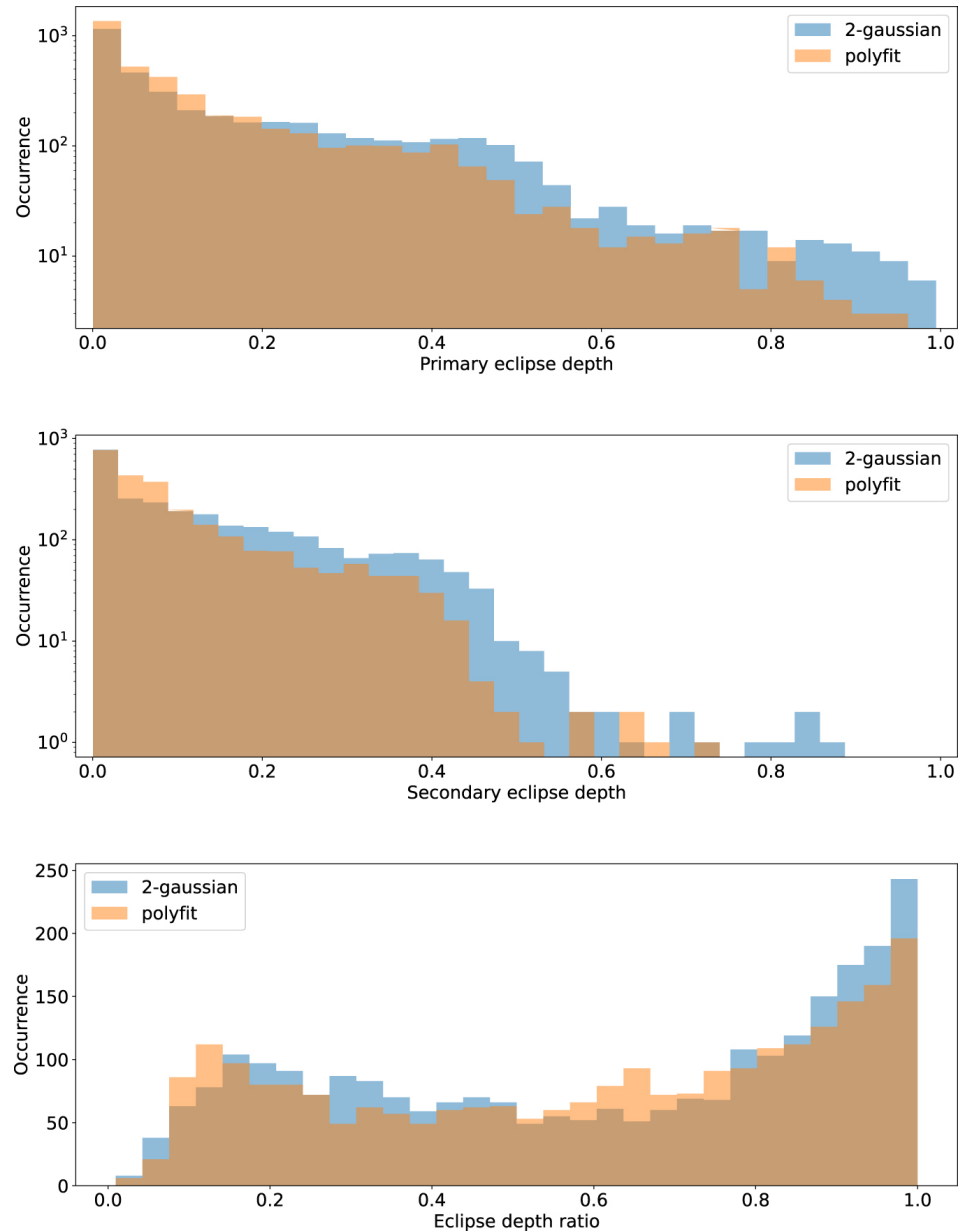
Figure 9. from TESS Eclipsing Binary Stars. I. Short-cadence Observations of 4584 Eclipsing Binaries in Sectors 1–26 null 2022 APJS 258 16 doi:10.3847/1538-4365/ac324a https://dx.doi.org/10.3847/1538-4365/ac324a © 2022. The Author(s). Published by the American Astronomical Society.
