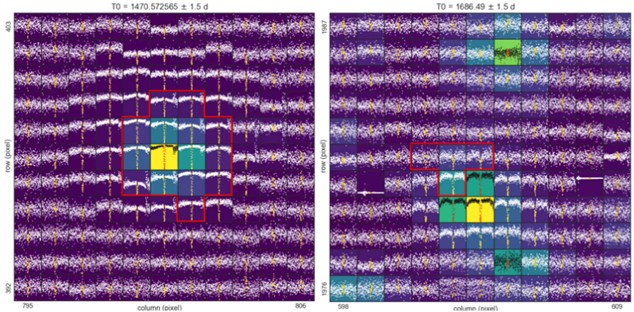
Figure 6. from TESS Eclipsing Binary Stars. I. Short-cadence Observations of 4584 Eclipsing Binaries in Sectors 1–26 null 2022 APJS 258 16 doi:10.3847/1538-4365/ac324a https://dx.doi.org/10.3847/1538-4365/ac324a © 2022. The Author(s). Published by the American Astronomical Society.
