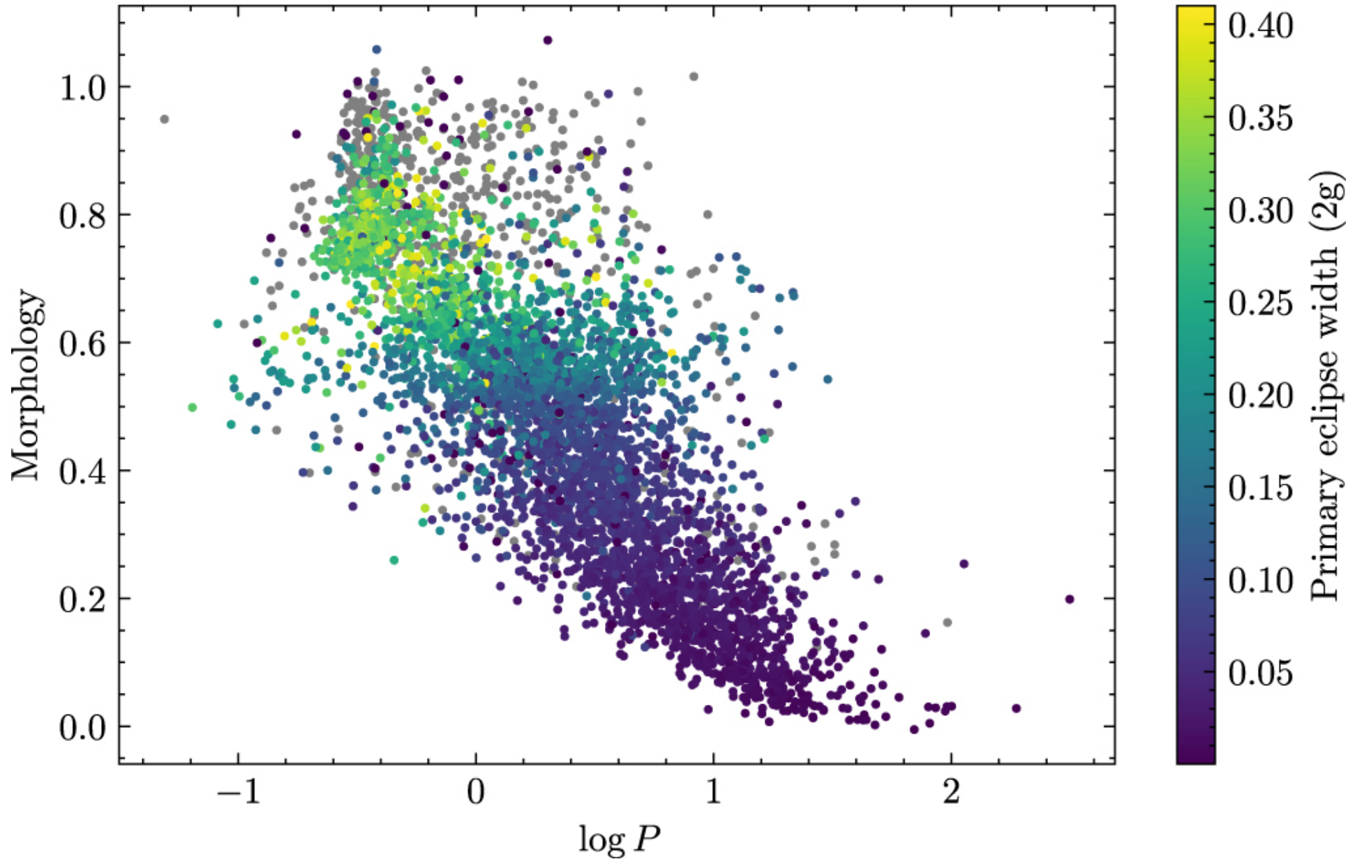
Figure 5. from TESS Eclipsing Binary Stars. I. Short-cadence Observations of 4584 Eclipsing Binaries in Sectors 1–26 null 2022 APJS 258 16 doi:10.3847/1538-4365/ac324a http://dx.doi.org/10.3847/1538-4365/ac324a © 2022. The Author(s). Published by the American Astronomical Society.
