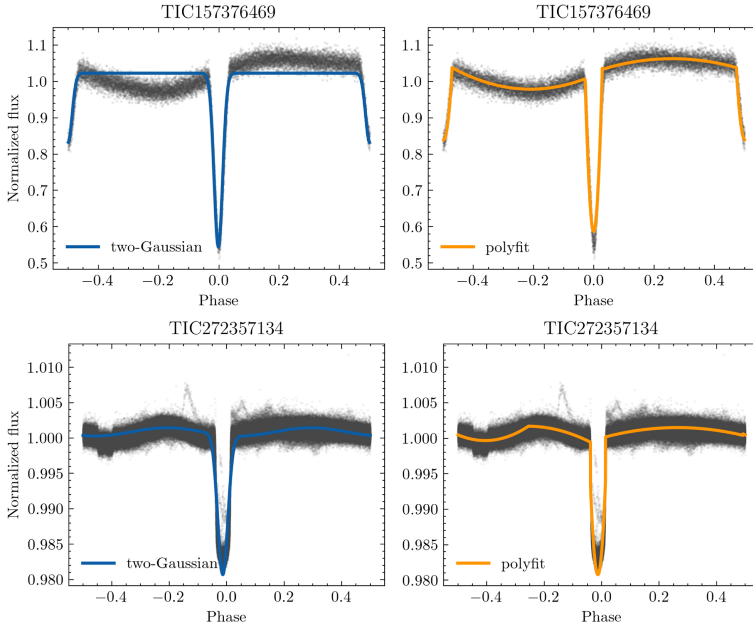
Figure 3. from TESS Eclipsing Binary Stars. I. Short-cadence Observations of 4584 Eclipsing Binaries in Sectors 1–26 null 2022 APJS 258 16 doi:10.3847/1538-4365/ac324a https://dx.doi.org/10.3847/1538-4365/ac324a © 2022. The Author(s). Published by the American Astronomical Society.
