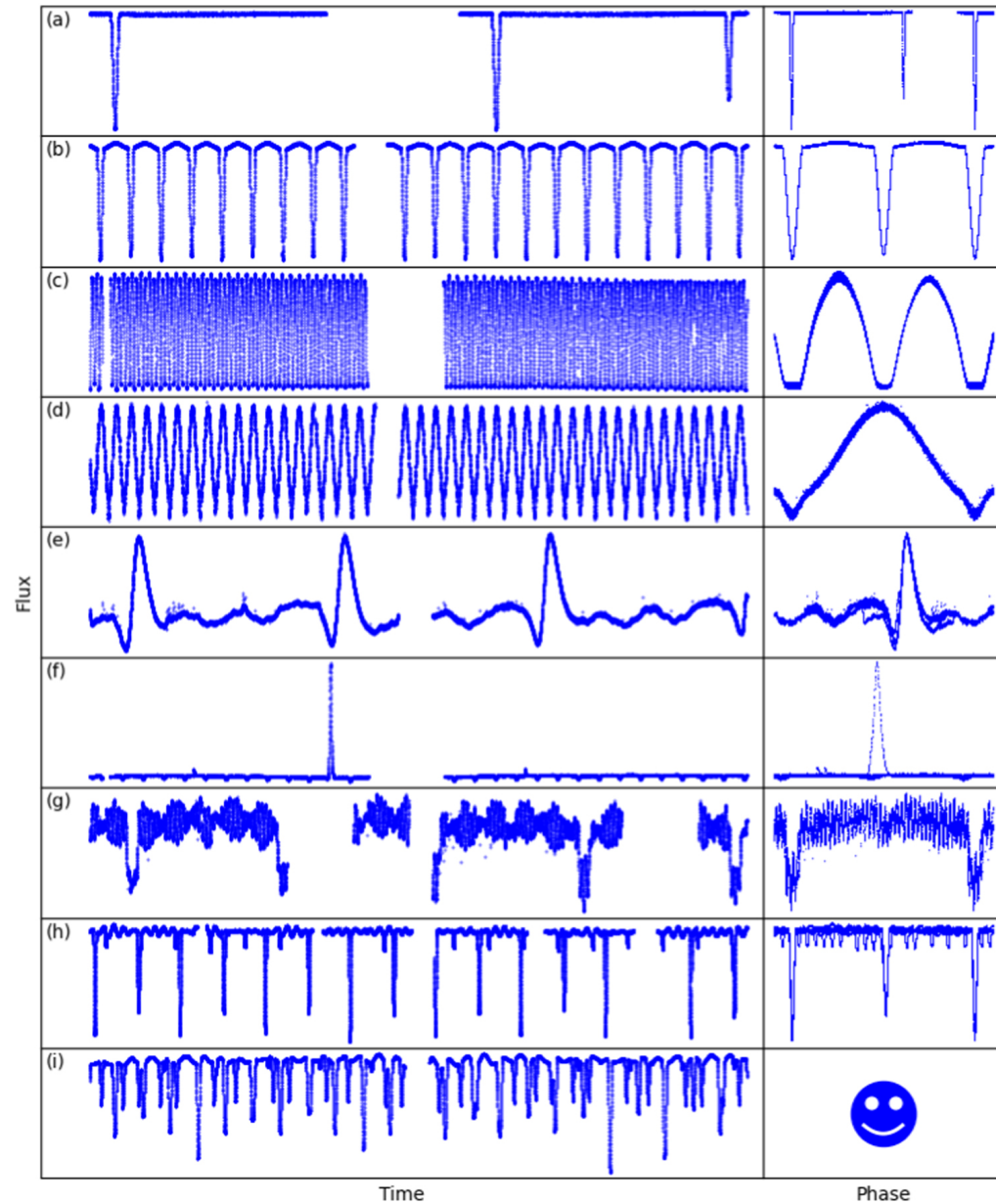
Figure 2. from TESS Eclipsing Binary Stars. I. Short-cadence Observations of 4584 Eclipsing Binaries in Sectors 1–26 null 2022 APJS 258 16 doi:10.3847/1538-4365/ac324a https://dx.doi.org/10.3847/1538-4365/ac324a © 2022. The Author(s). Published by the American Astronomical Society.
