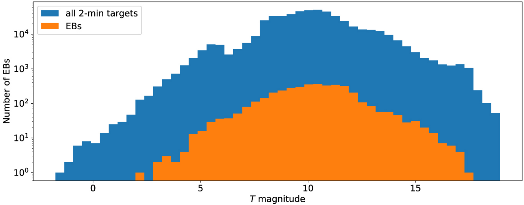
Figure 14. from TESS Eclipsing Binary Stars. I. Short-cadence Observations of 4584 Eclipsing Binaries in Sectors 1–26 null 2022 APJS 258 16 doi:10.3847/1538-4365/ac324a http://dx.doi.org/10.3847/1538-4365/ac324a © 2022. The Author(s). Published by the American Astronomical Society.
