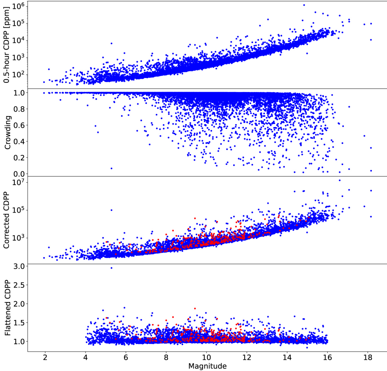
Figure 12. from TESS Eclipsing Binary Stars. I. Short-cadence Observations of 4584 Eclipsing Binaries in Sectors 1–26 null 2022 APJS 258 16 doi:10.3847/1538-4365/ac324a http://dx.doi.org/10.3847/1538-4365/ac324a © 2022. The Author(s). Published by the American Astronomical Society.
