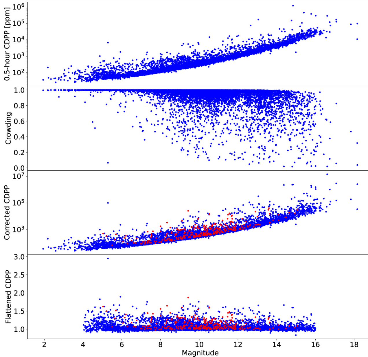
Figure 12. from TESS Eclipsing Binary Stars. I. Short-cadence Observations of 4584 Eclipsing Binaries in Sectors 1–26 null 2022 APJS 258 16 doi:10.3847/1538-4365/ac324a https://dx.doi.org/10.3847/1538-4365/ac324a © 2022. The Author(s). Published by the American Astronomical Society.
