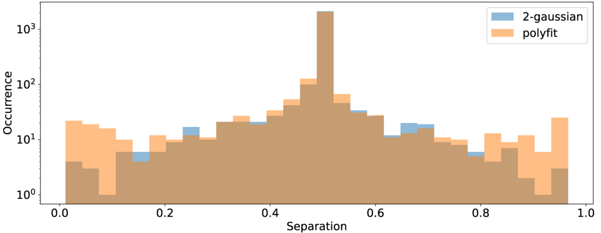
Figure 10. from TESS Eclipsing Binary Stars. I. Short-cadence Observations of 4584 Eclipsing Binaries in Sectors 1–26 null 2022 APJS 258 16 doi:10.3847/1538-4365/ac324a http://dx.doi.org/10.3847/1538-4365/ac324a © 2022. The Author(s). Published by the American Astronomical Society.
