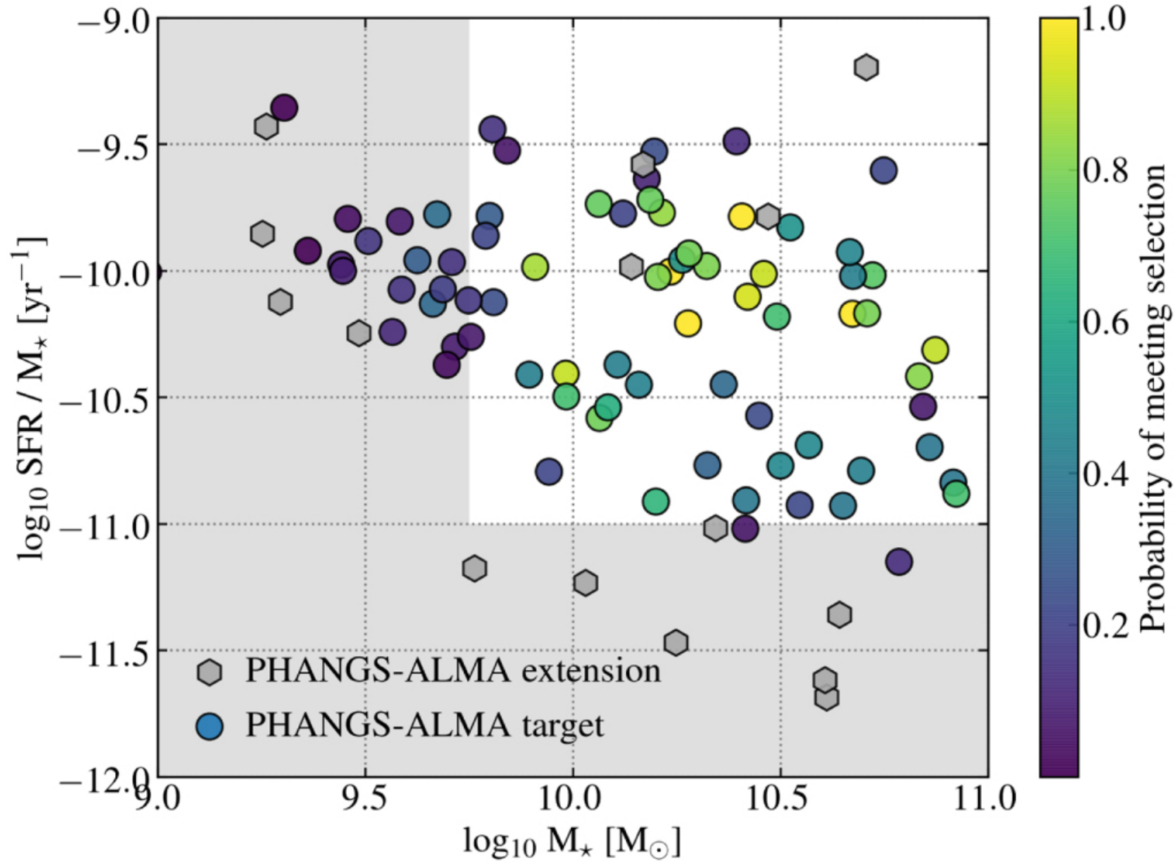
Figure 7. from PHANGS–ALMA: Arcsecond CO(2–1) Imaging of Nearby Star-forming Galaxies null 2021 APJS 257 43 doi:10.3847/1538-4365/ac17f3 http://dx.doi.org/10.3847/1538-4365/ac17f3 © 2021. The American Astronomical Society. All rights reserved.
