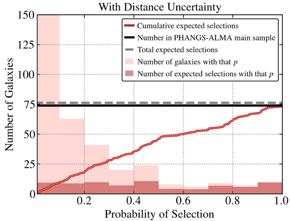
Figure 5. from PHANGS–ALMA: Arcsecond CO(2–1) Imaging of Nearby Star-forming Galaxies null 2021 APJS 257 43 doi:10.3847/1538-4365/ac17f3 http://dx.doi.org/10.3847/1538-4365/ac17f3 © 2021. The American Astronomical Society. All rights reserved.
