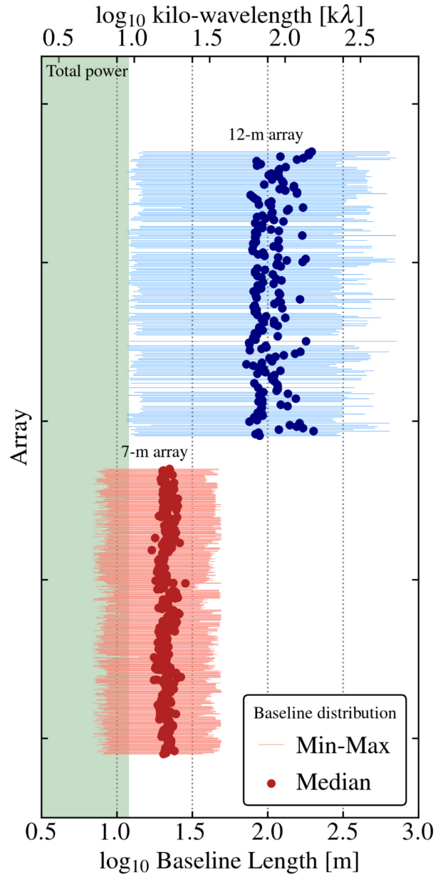
Figure 23. from PHANGS–ALMA: Arcsecond CO(2–1) Imaging of Nearby Star-forming Galaxies null 2021 APJS 257 43 doi:10.3847/1538-4365/ac17f3 http://dx.doi.org/10.3847/1538-4365/ac17f3 © 2021. The American Astronomical Society. All rights reserved.
