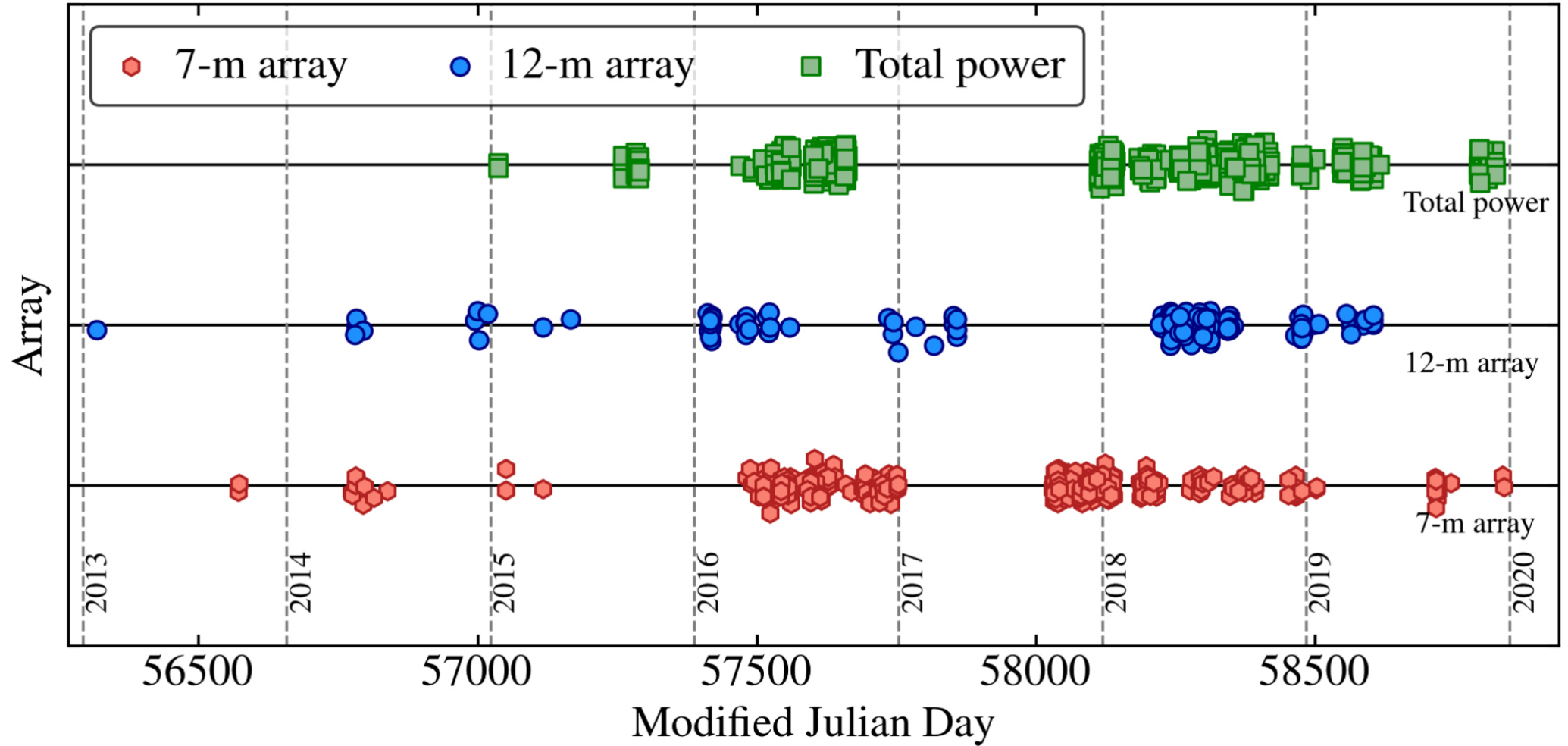
Figure 21. from PHANGS–ALMA: Arcsecond CO(2–1) Imaging of Nearby Star-forming Galaxies null 2021 APJS 257 43 doi:10.3847/1538-4365/ac17f3 http://dx.doi.org/10.3847/1538-4365/ac17f3 © 2021. The American Astronomical Society. All rights reserved.
