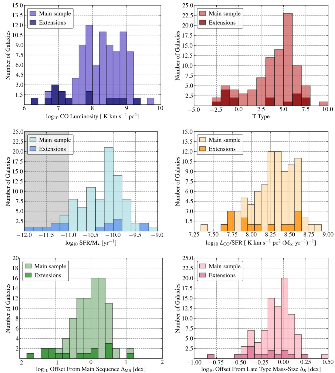
Figure 17. from Adam K. Leroy et al 2021 Astrophys. J. Suppl. 257 doi:10.3847/1538-4365/ac17f3 https://dx.doi.org/10.3847/1538-4365/ac17f3 © 2021. The American Astronomical Society. All rights reserved.
