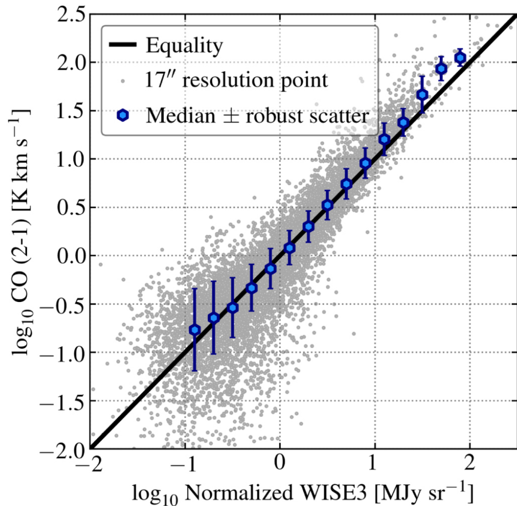
Figure 14. from PHANGS–ALMA: Arcsecond CO(2–1) Imaging of Nearby Star-forming Galaxies null 2021 APJS 257 43 doi:10.3847/1538-4365/ac17f3 http://dx.doi.org/10.3847/1538-4365/ac17f3 © 2021. The American Astronomical Society. All rights reserved.
