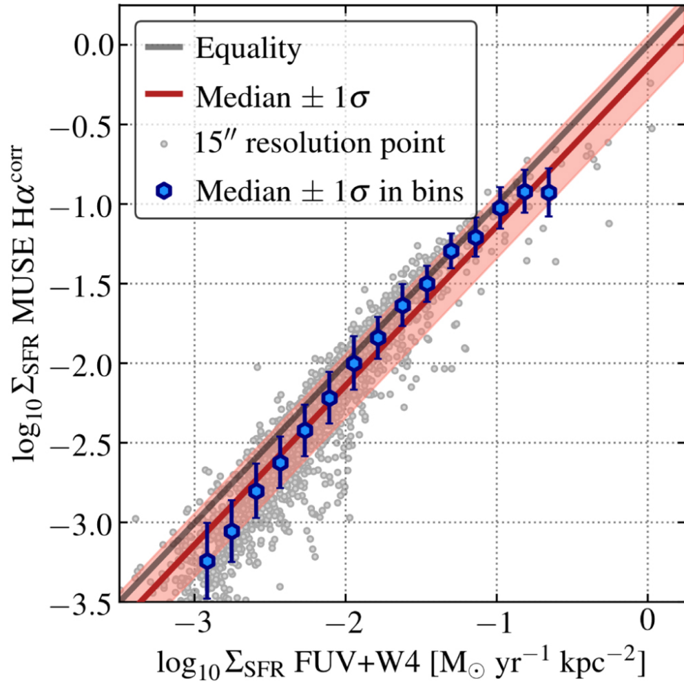
Figure 13. from PHANGS–ALMA: Arcsecond CO(2–1) Imaging of Nearby Star-forming Galaxies null 2021 APJS 257 43 doi:10.3847/1538-4365/ac17f3 http://dx.doi.org/10.3847/1538-4365/ac17f3 © 2021. The American Astronomical Society. All rights reserved.
