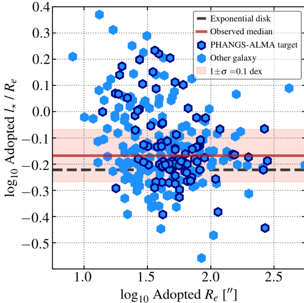
Figure 11. from PHANGS–ALMA: Arcsecond CO(2–1) Imaging of Nearby Star-forming Galaxies null 2021 APJS 257 43 doi:10.3847/1538-4365/ac17f3 http://dx.doi.org/10.3847/1538-4365/ac17f3 © 2021. The American Astronomical Society. All rights reserved.
