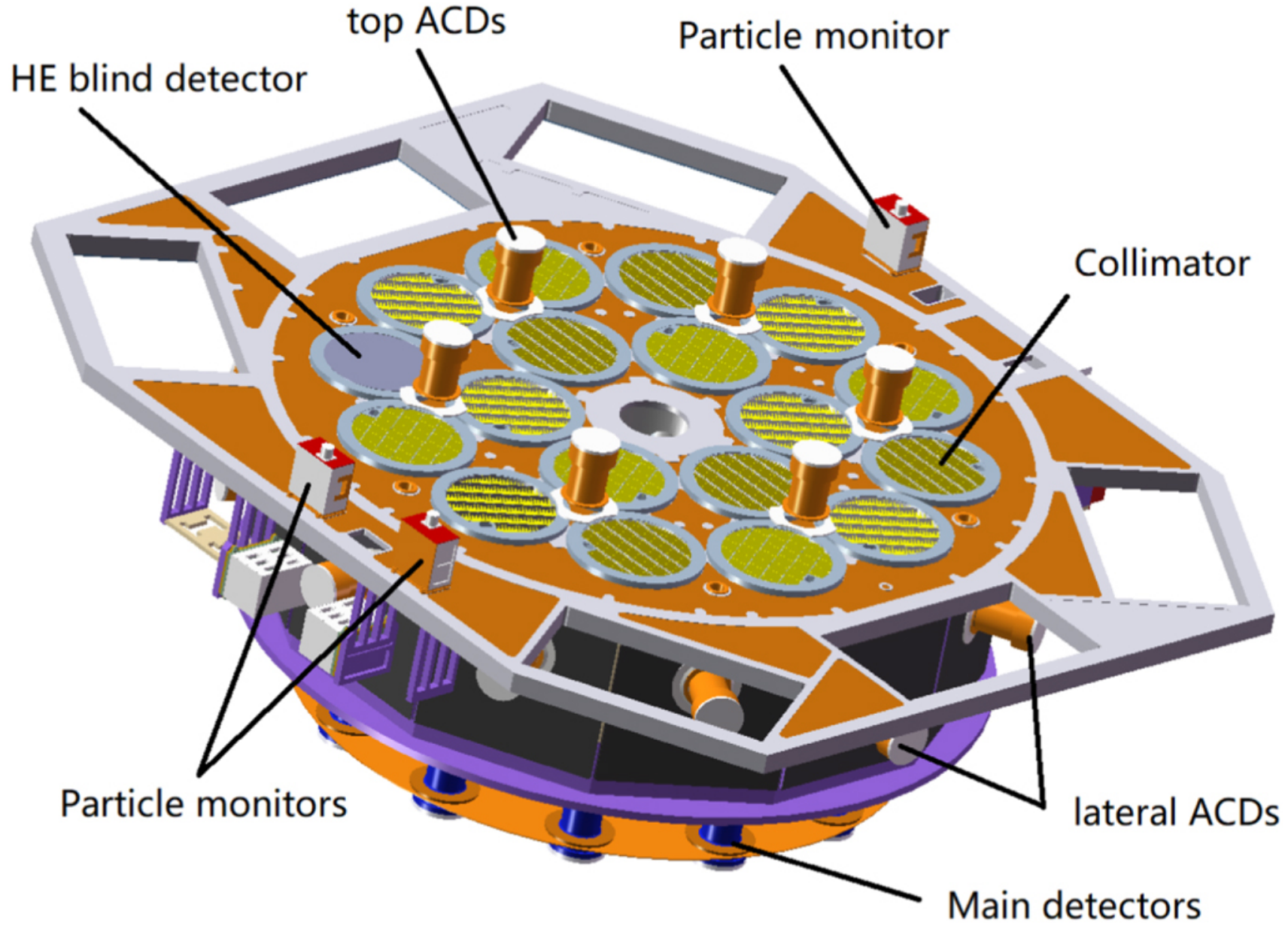
Figure 1. from A Parametric Model to Reproduce the Background of the Insight-HXMT/HE Blind Detector null 2021 APJS 256 47 doi:10.3847/1538-4365/ac16db http://dx.doi.org/10.3847/1538-4365/ac16db © 2021. The American Astronomical Society. All rights reserved.
