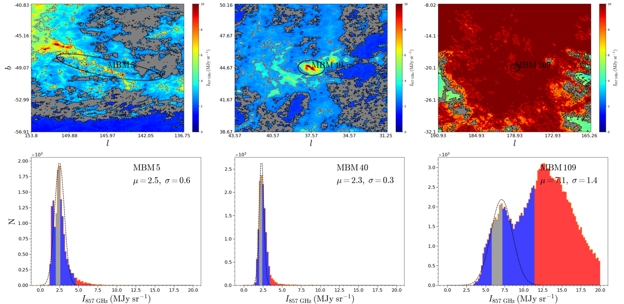
Figure 3. from Mingxu Sun et al 2021 Astrophys. J. Suppl. 256 doi:10.3847/1538-4365/ac1601 https://dx.doi.org/10.3847/1538-4365/ac1601 © 2021. The Author(s). Published by the American Astronomical Society.
